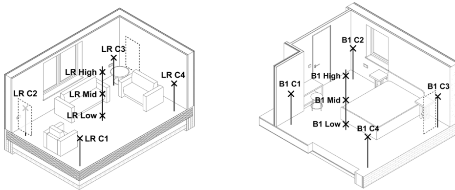
Figure 18. The Future Home Living Room (left) and Bedroom 1 (right) temperature measurement locations
