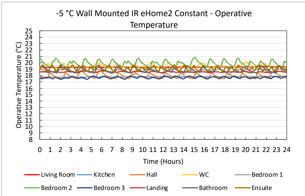
Figure 127. -5 °C Wall Mounted IR eHome2 Constant – Operative Temperature Plots
