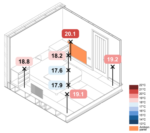
-5°C Wall Mounted IR TFH Constant – Operative - 7h
