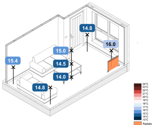
Figure 65. -5 °C Monobloc ASHP TFH Rads SAP – Spatial Operative Temperatures
