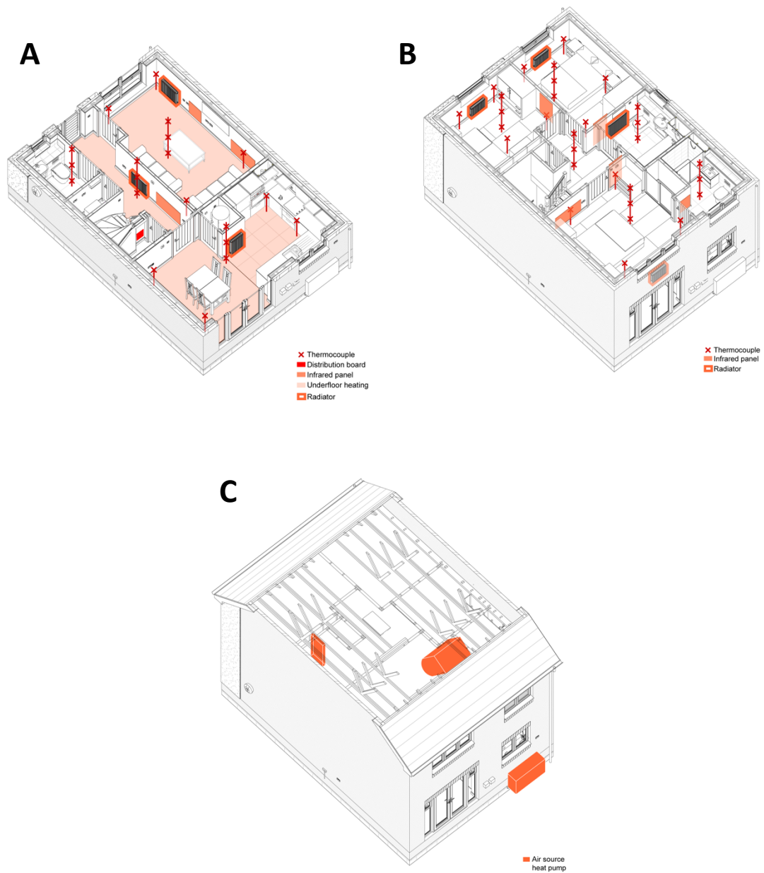
Figure 15. Heating systems and emitters in TFH. A) Radiators and UFH. B) IR Panels. C) Loft and Monobloc ASHPs.
