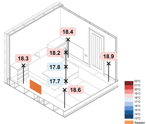
Figure 41. -5 °C Loft ASHP Rads Constant - Spatial Air Temperatures
