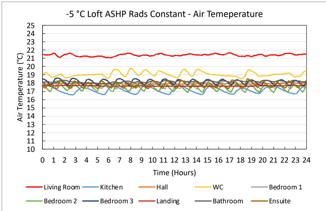
Figure 38. -5 °C Loft ASHP Rads Constant – Air Temperature Plots
