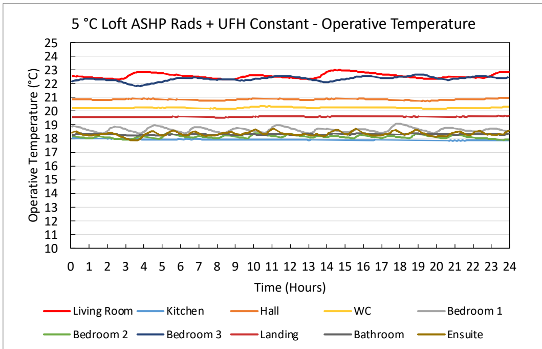
Figure 77. 5 °C Loft ASHP Rads + UFH Constant – Operative Temperature Plots
