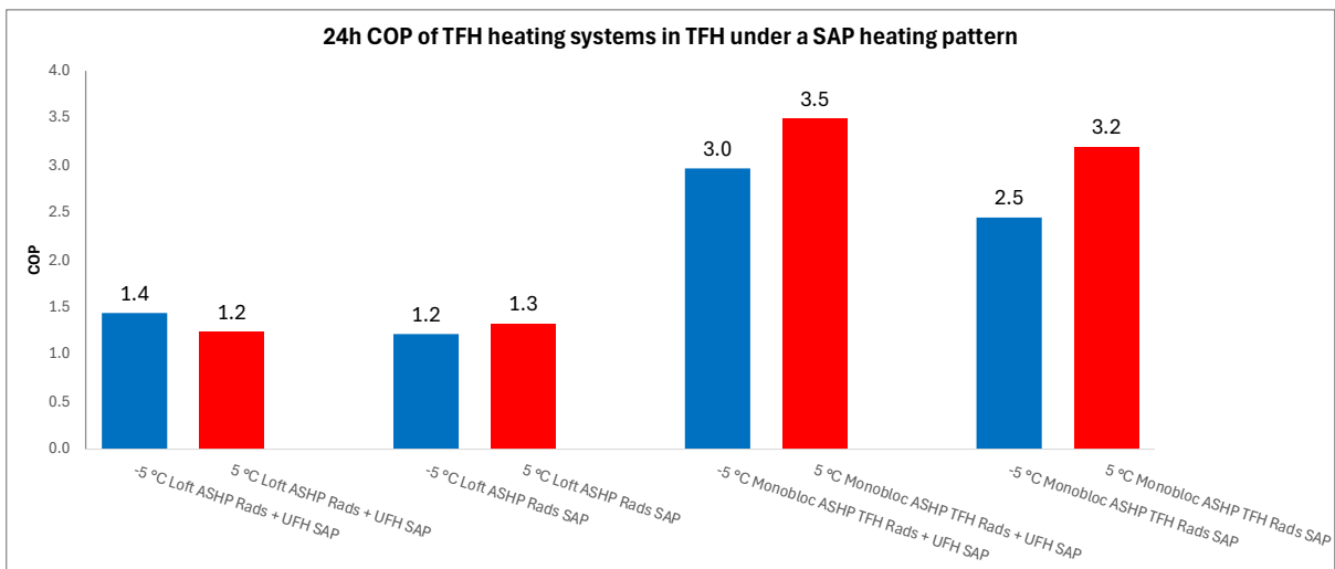
Figure 153. 24h COP of TFH heating systems under a SAP heating pattern
