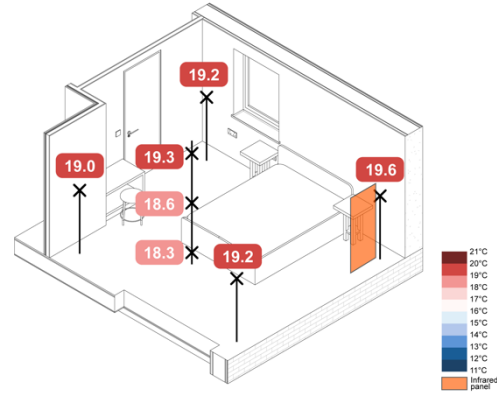
Figure 147. 5 °C Wall Mounted eHome2 Constant – Spatial Air Temperatures
