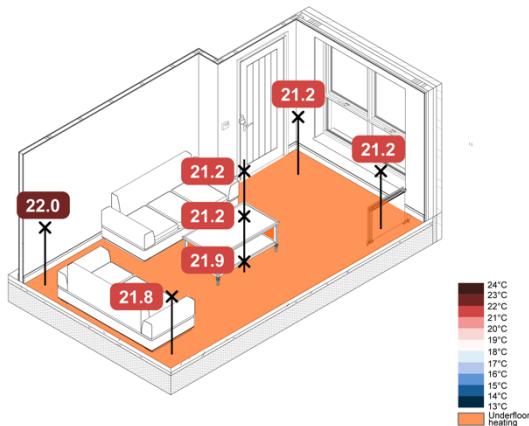
Figure 55. -5 °C Monobloc ASHP TFH Rads + UFH SAP – Spatial Operative Temperatures
