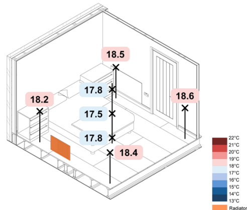
Figure 50. -5 °C Monobloc ASHP TFH Rads + UFH Constant – Spatial Operative Temperatures
