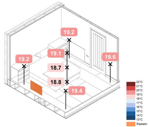
Figure 88. 5 °C Loft ASHP Rads Constant – Spatial Air Temperatures
