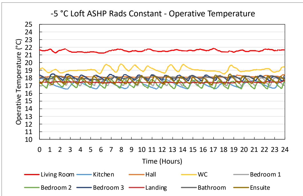
Figure 39. -5 °C Loft ASHP Rads Constant – Operative Temperature Plots
