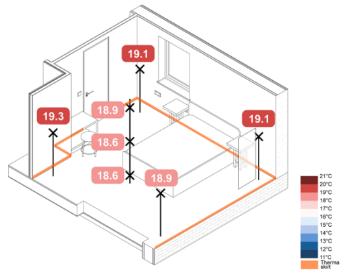
Figure 136. 5 °C Monobloc ASHP eHome2 Constant – Operative Temperature Plots
