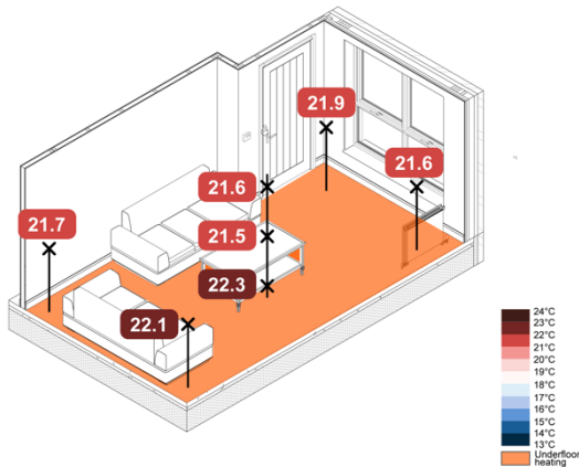
Figure 56. -5 °C Monobloc ASHP TFH Rads + UFH SAP – Spatial Air Temperatures
