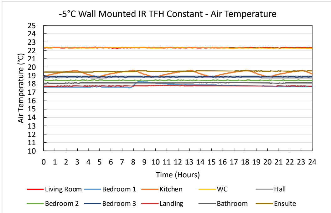
Figure 20. -5°C Wall Mounted IR TFH Constant Air Temperature Plot
