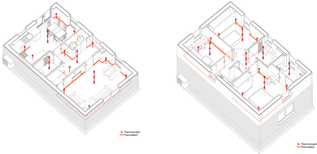
Figure 16. Heating emitters in eHome2 downstairs (left) and upstairs (right)
