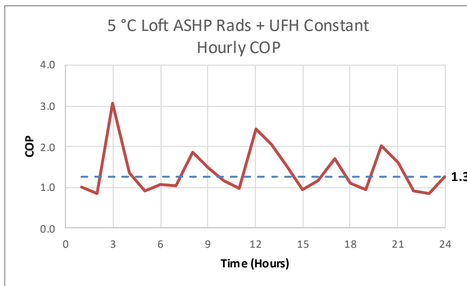
Figure 80. 5 °C Loft ASHP Rads + UFH Constant – Hourly COP
