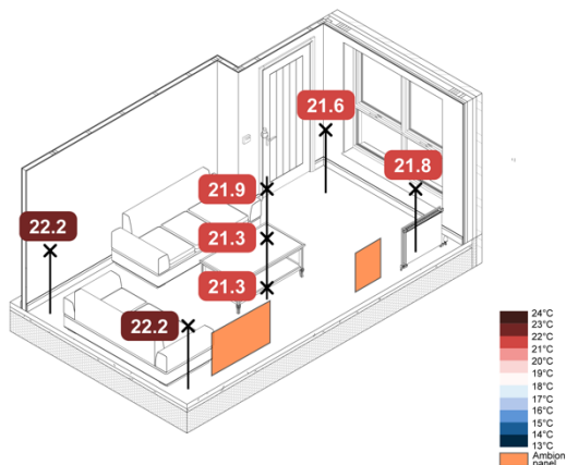
Figure 71. 5°C Wall Mounted IR TFH Constant – Spatial Operative Temperatures
