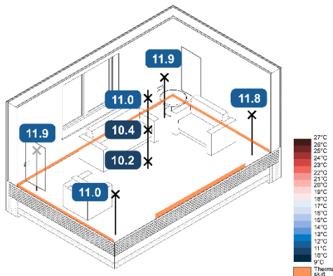
-5 °C Monobloc ASHP eHome2 SAP – Operative - 7h
