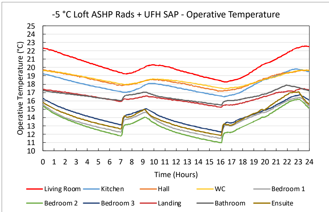
Figure 34. -5°C Loft ASHP Rads + UFH SAP – Operative Temperature Plots
