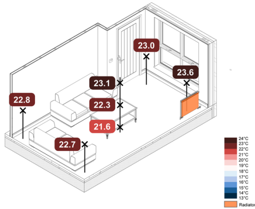
Figure 88. 5 °C Loft ASHP Rads Constant – Spatial Air Temperatures
