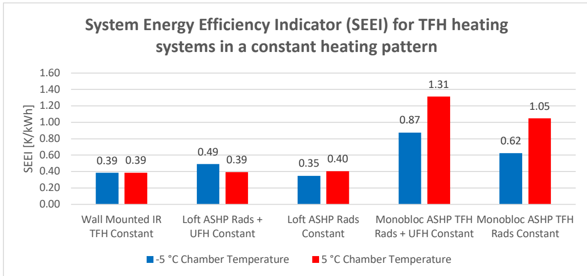
Figure 160. System Energy Efficiency Indicator (SEEI) for TFH heating system in a constant heating pattern
