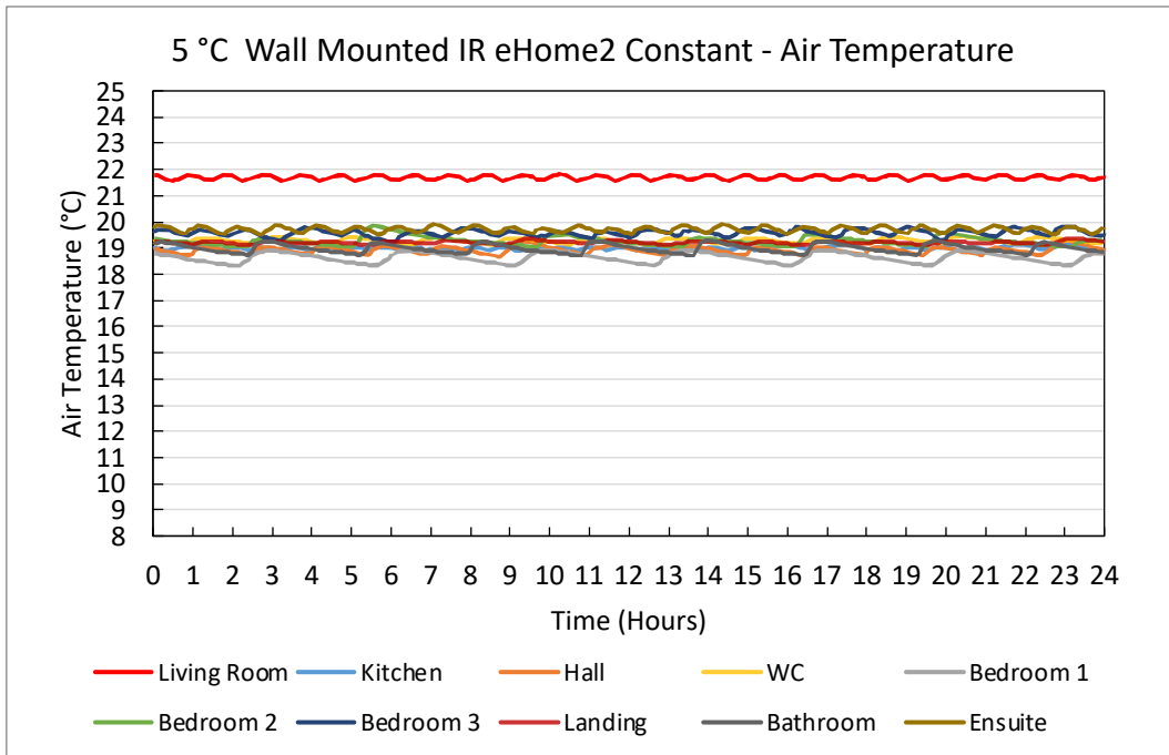
Figure 144. 5 °C Wall Mounted eHome2 Constant – Air Temperature Plots
