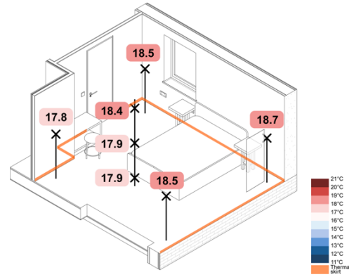
Figure 142. 5 °C Monobloc ASHP eHome2 SAP – Spatial Air Temperatures
