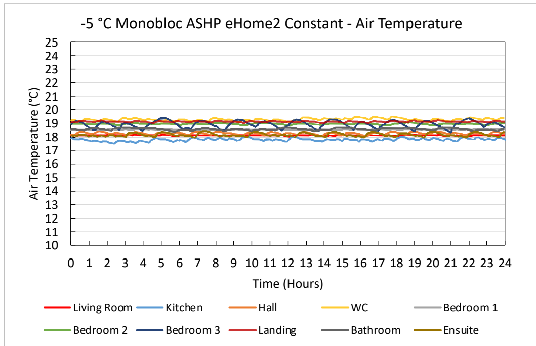
Figure 116. -5 °C Monobloc ASHP eHome2 Constant – Air Temperature Plots
