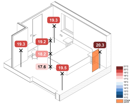
Figure 151. 5 °C Wall Mounted eHome2 SAP – Spatial Operative Temperatures
