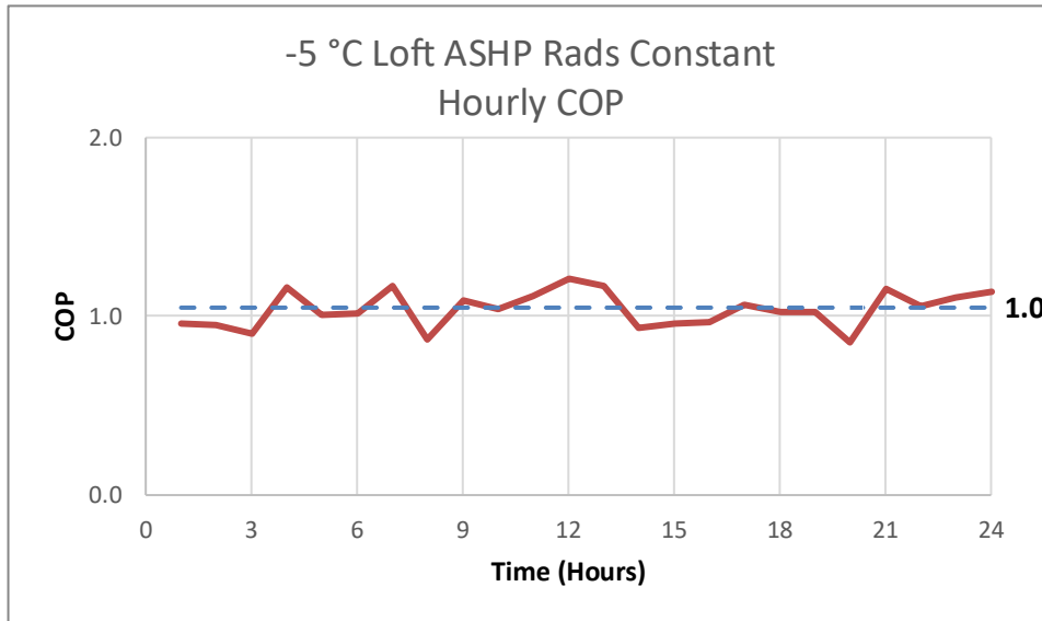
Figure 42. -5 °C Loft ASHP Rads Constant – Hourly COP
