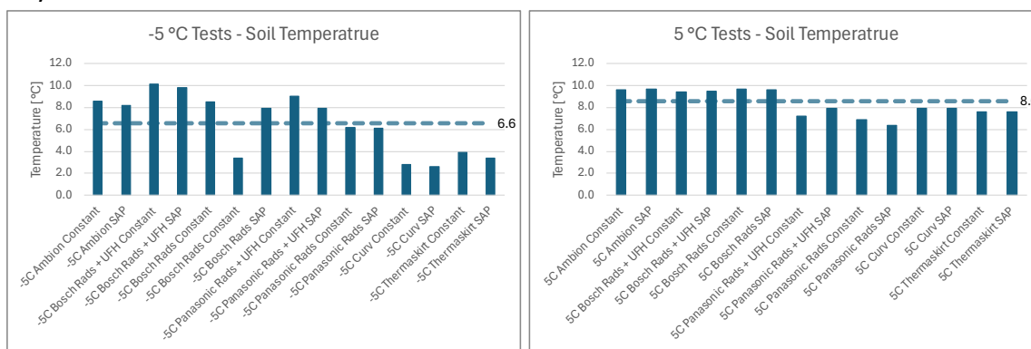
Figure 164. Soil Temperatures in -5 °C and 5 °C tests
