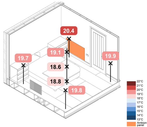
Figure 70. 5°C Wall Mounted IR TFH Constant – Spatial Air Temperatures
