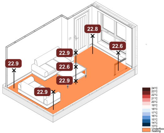
Figure 51. -5 °C Monobloc ASHP TFH Rads + UFH Constant – Spatial Air Temperatures
