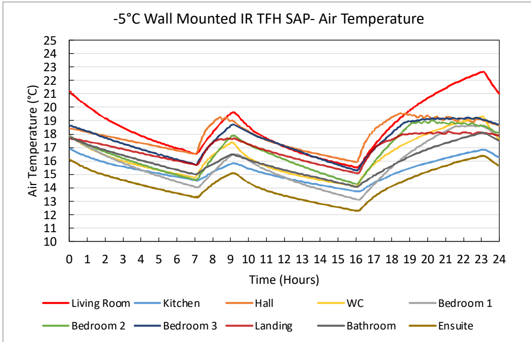
Figure 24. -5°C Wall Mounted IR TFH SAP - Air Temperature Plots
