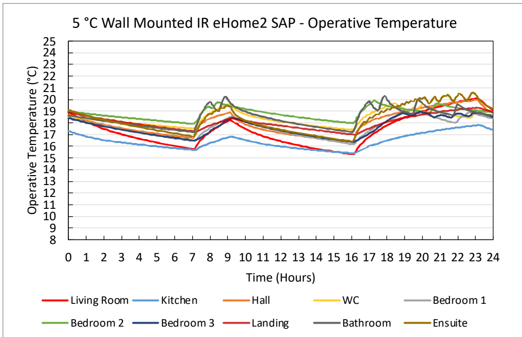
Figure 149. 5 °C Wall Mounted eHome2 SAP – Operative Temperature Plots
