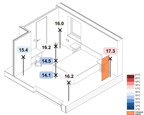
Figure 132. -5 °C Wall Mounted IR eHome2 SAP – Spatial Air Temperatures
