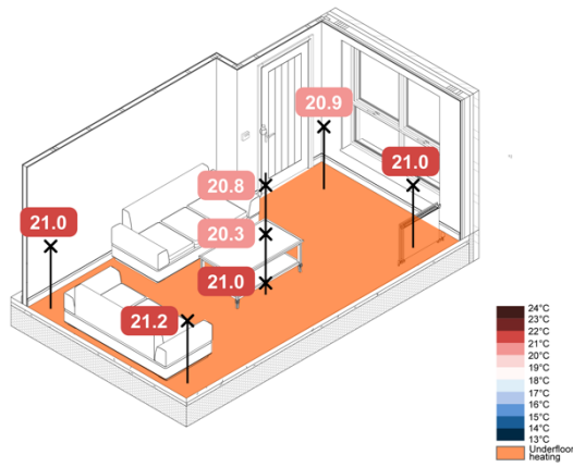
Figure 35. -5°C Loft ASHP Rads + UFH SAP – Spatial Air Temperatures
