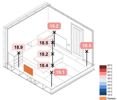
Figure 31. -5°C Loft ASHP Rads + UFH Constant - Spatial Operative Temperature Plots
