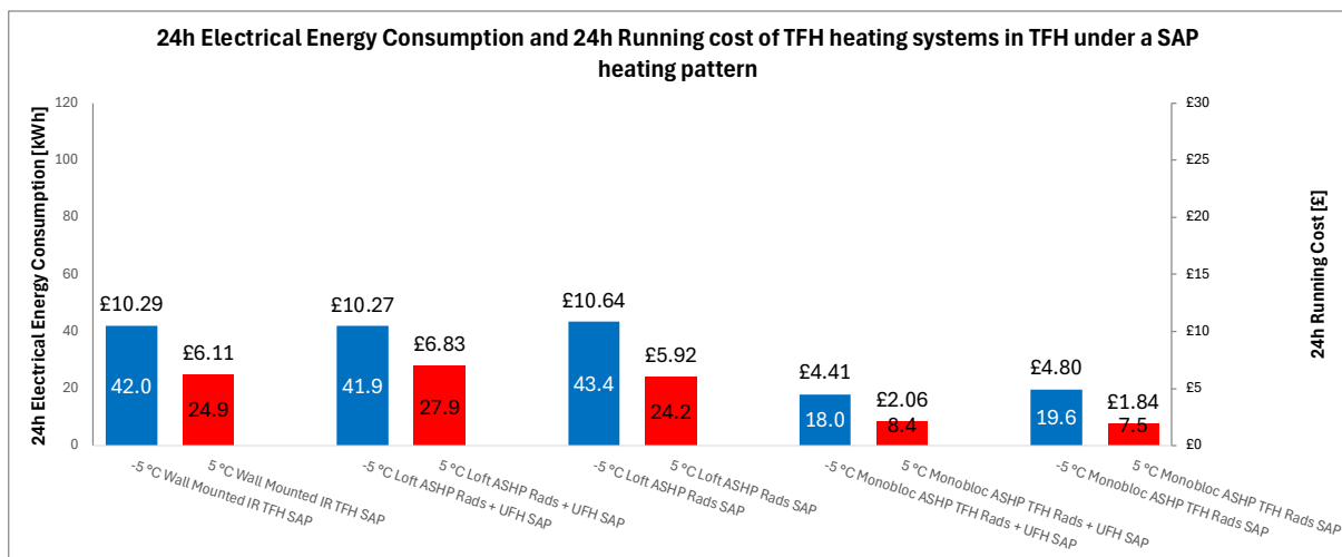
Figure 157. 24h Electrical Energy Consumption and 24h Running Cost of TFH heating system under a SAP heating pattern
