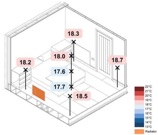
Figure 61. -5 °C Monobloc ASHP TFH Rads Constant – Spatial Air Temperatures
