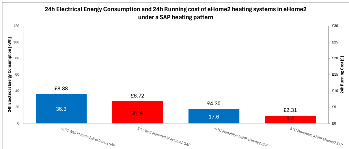
Figure 159. 24h Electrical Energy Consumption and 24h Running Cost of eHome2 heating system under a SAP heating pattern
