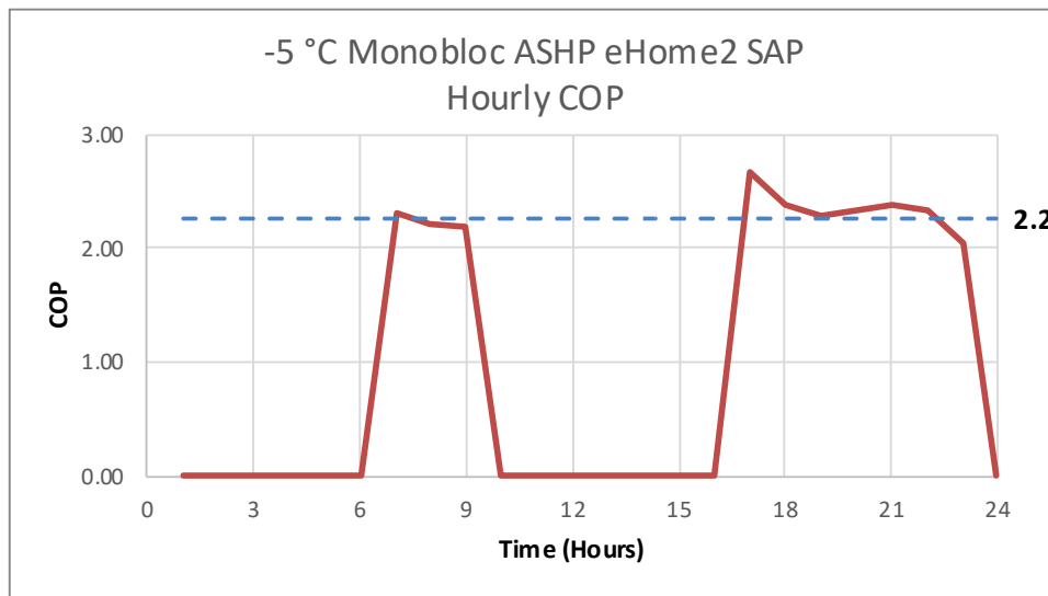
Figure 125. -5 °C Monobloc ASHP eHome2 SAP – Hourly COP
