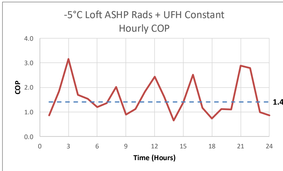
Figure 32. -5°C Loft ASHP Rads + UFH Constant – Hourly COP
