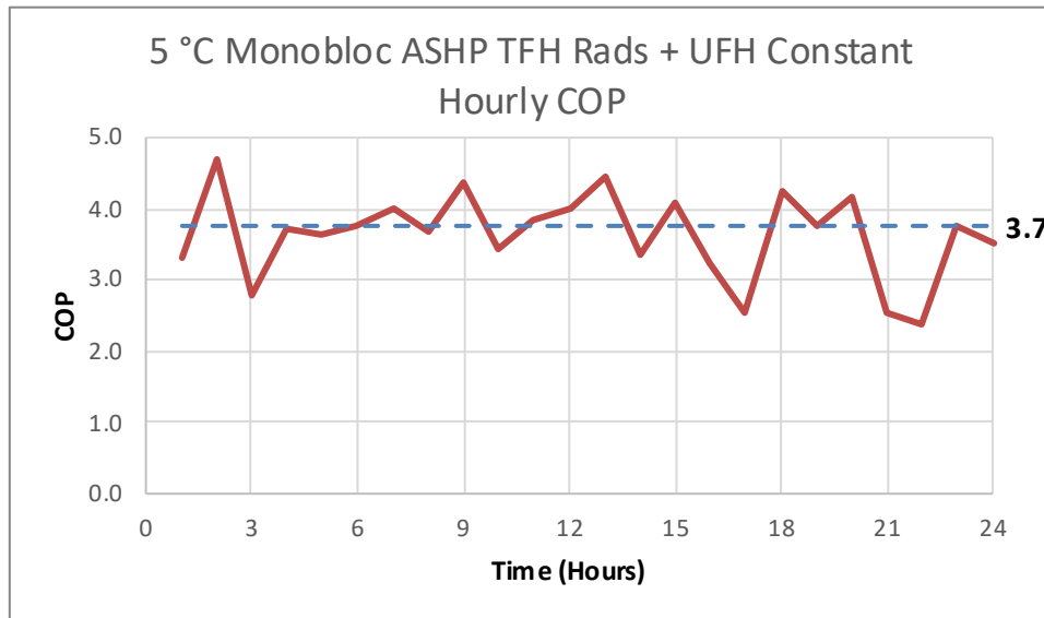
Figure 100. 5 °C Monobloc ASHP TFH Rads + UFH Constant – Hourly COP
