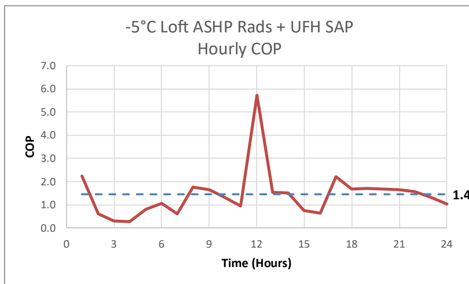
Figure 37. -5°C Loft ASHP Rads + UFH SAP – Hourly COP
