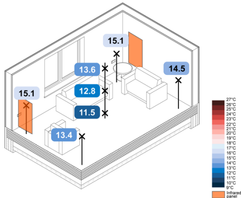
Figure 132. -5 °C Wall Mounted IR eHome2 SAP – Spatial Air Temperatures
