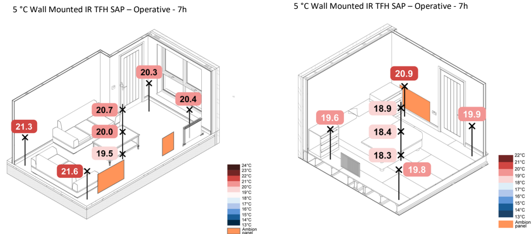
Figure 74. 5 °C Wall Mounted IR TFH SAP – Spatial Operative Temperatures
