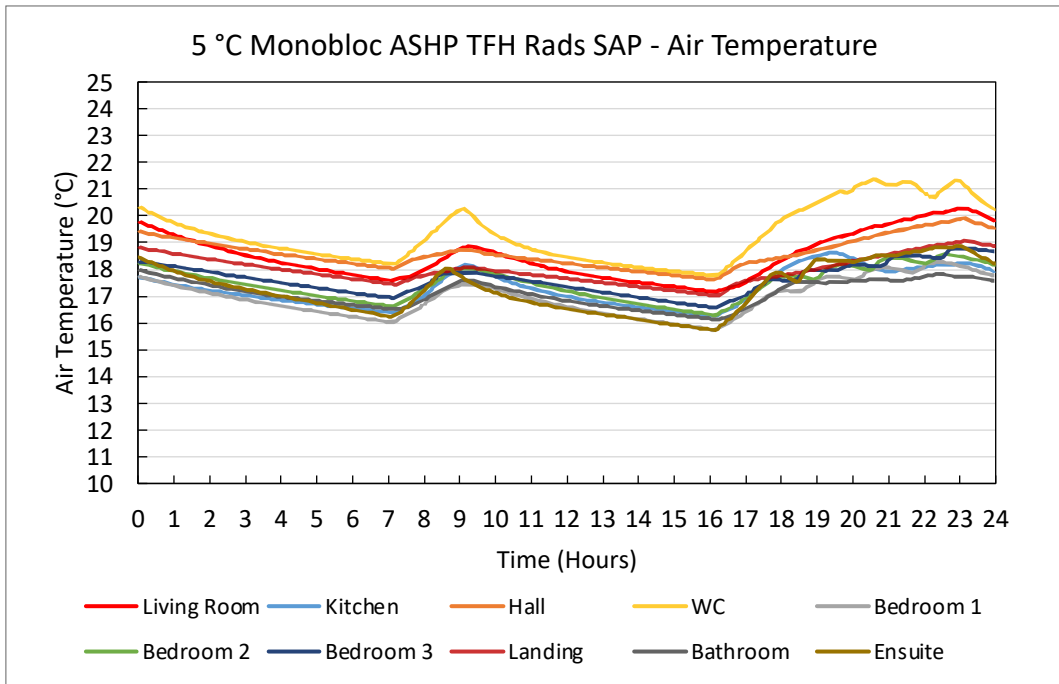
Figure 111. 5 °C Monobloc ASHP TFH Rads SAP – Air Temperature Plots
