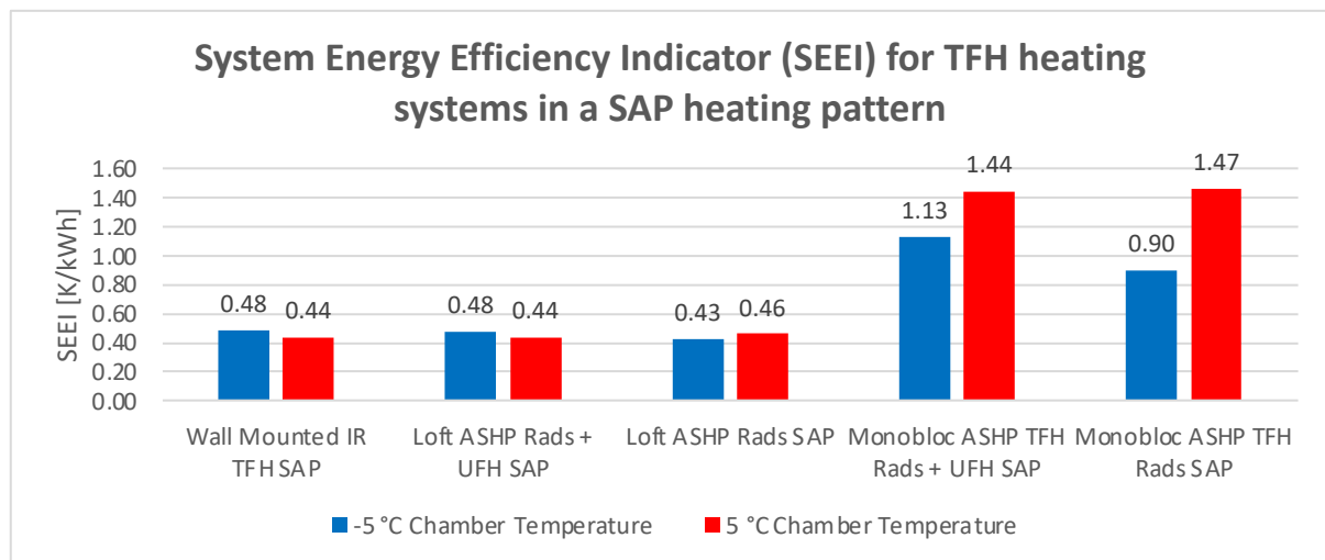
Figure 161. System Energy Efficiency Indicator (SEEI) for TFH heating system in a SAP heating pattern
