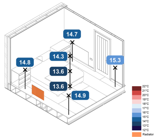
Figure 66. -5 °C Monobloc ASHP TFH Rads SAP – Spatial Air Temperatures
