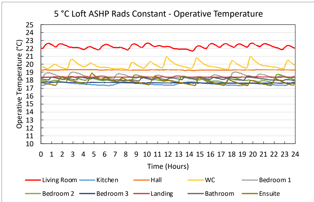
Figure 87. 5 °C Loft ASHP Rads Constant – Operative Temperature Plots
