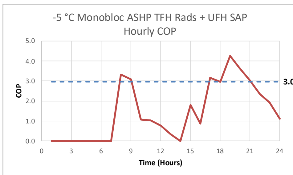
Figure 57. -5 °C Monobloc ASHP TFH Rads + UFH SAP – Hourly COP
