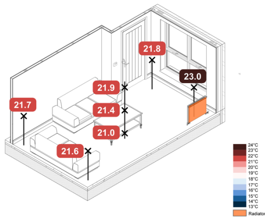
Figure 41. -5 °C Loft ASHP Rads Constant - Spatial Air Temperatures
