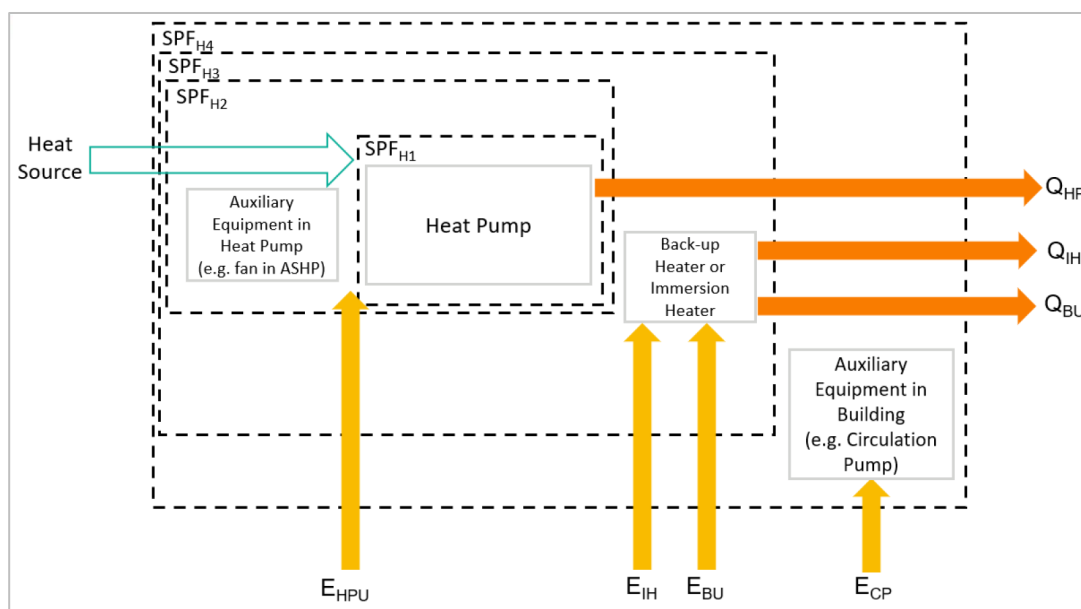
Figure 19. SPF system boundaries used to calculate coefficient of performance (COP) values. Test conditions meant that the immersion heater ( E_{IH} and Q_{IH} ) was not used in the systems tests at Energy House 2.0. 2
