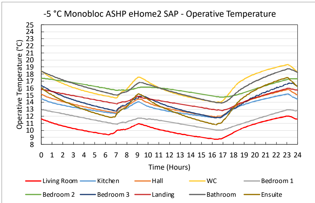
Figure 122. -5 °C Monobloc ASHP eHome2 SAP – Operative Temperature Plots
