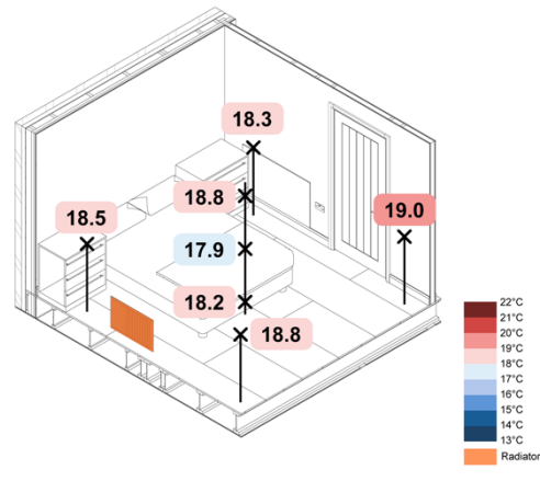
Figure 93. 5 °C Loft ASHP Rads SAP – Spatial Operative Temperatures
