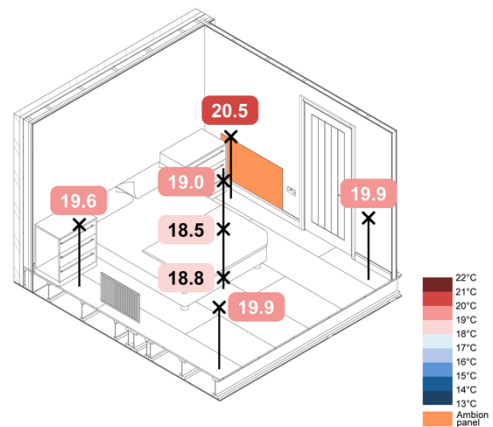
Figure 71. 5°C Wall Mounted IR TFH Constant – Spatial Operative Temperatures
