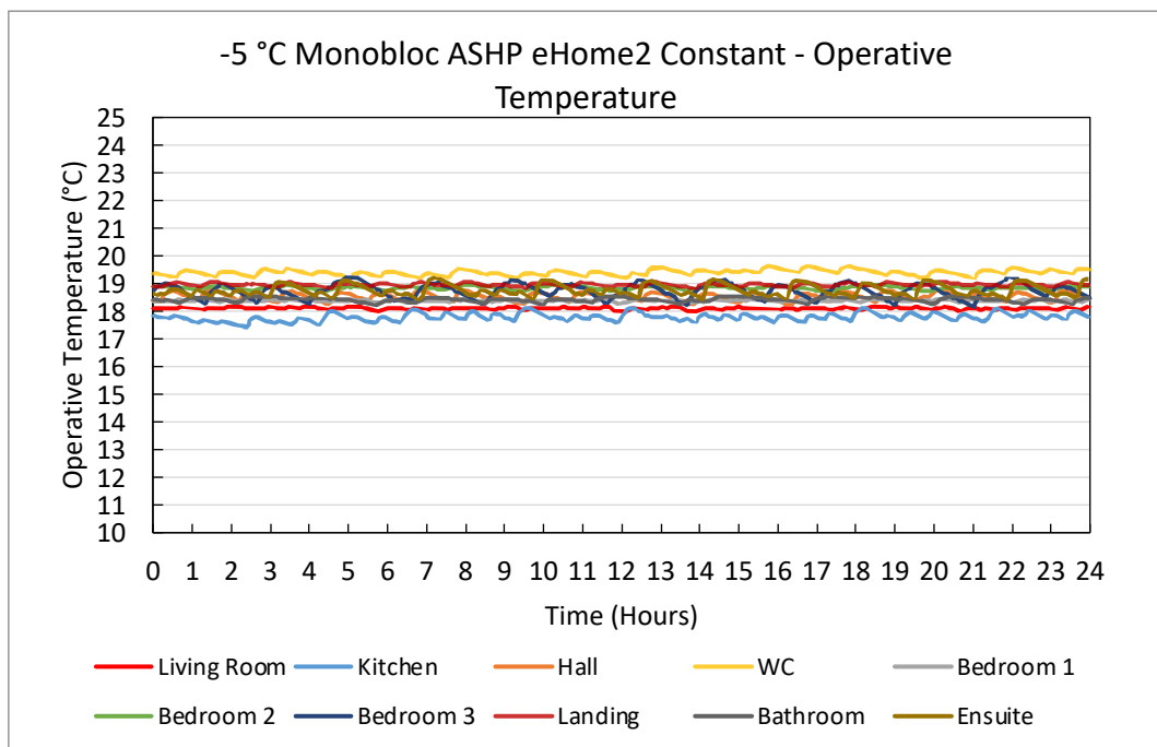
Figure 117. -5 °C Monobloc ASHP eHome2 Constant – Operative Temperature Plots
