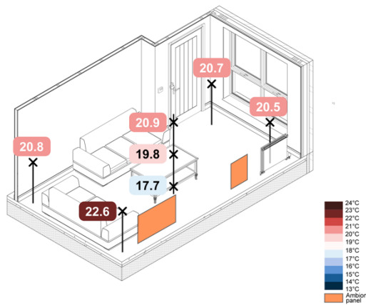
-5°C Wall Mounted IR TFH SAP – Air - 7h
