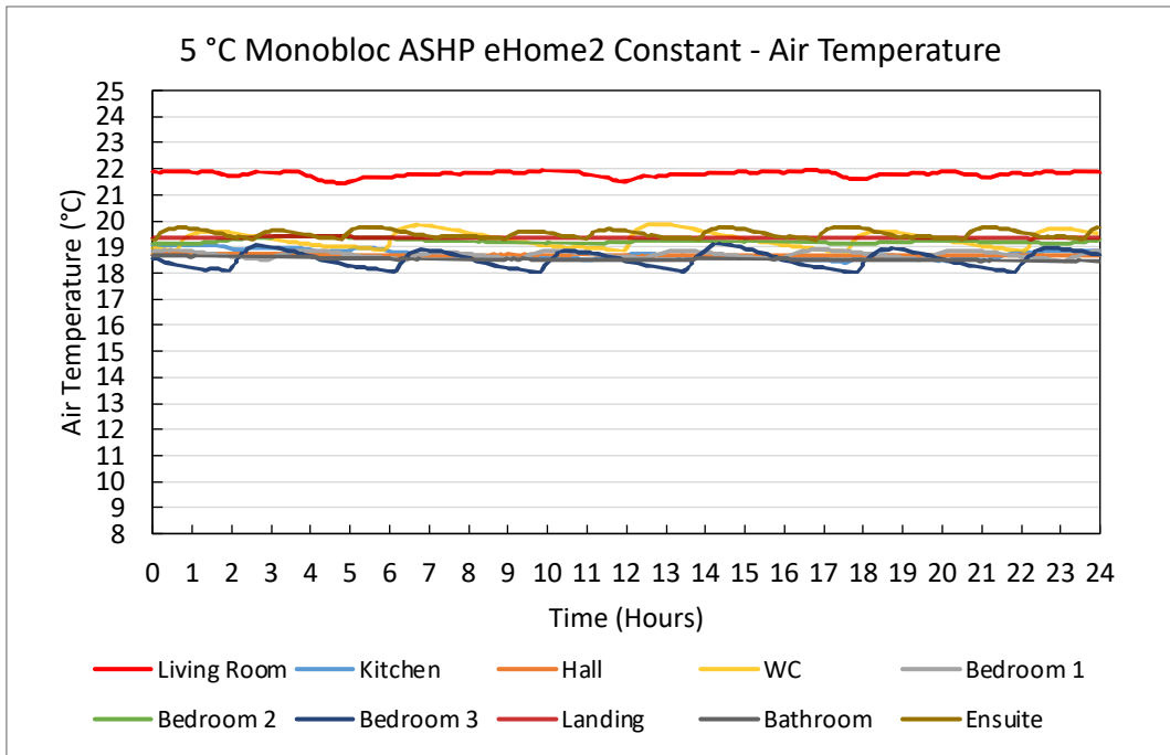
Figure 134. 5 °C Monobloc ASHP eHome2 Constant – Air Temperature Plots
