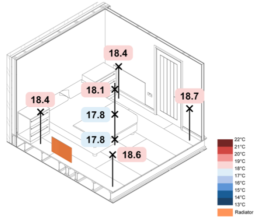
Figure 51. -5 °C Monobloc ASHP TFH Rads + UFH Constant – Spatial Air Temperatures
