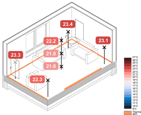
Figure 137. 5 °C Monobloc ASHP eHome2 Constant – Spatial Air Temperatures
