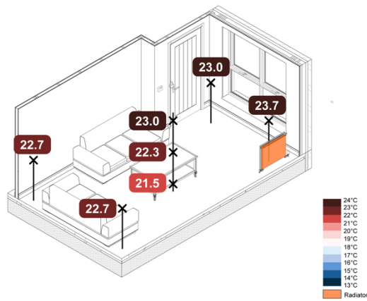
Figure 109. 5 °C Monobloc ASHP TFH Rads Constant – Spatial Air Temperatures
