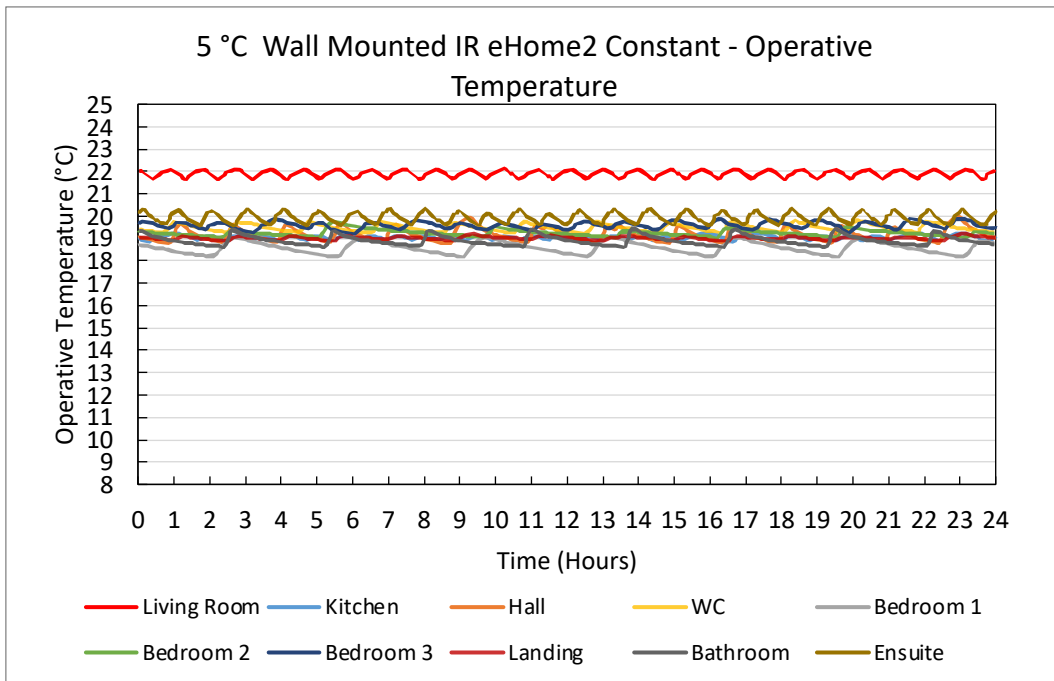
Figure 145. 5 °C Wall Mounted eHome2 Constant – Operative Temperature Plots
