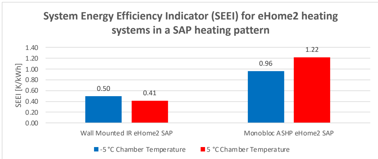
Figure 163. System Energy Efficiency Indicator (SEEI) for eHome2 heating system in a SAP heating pattern
