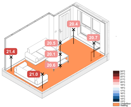
Figure 36. -5°C Loft ASHP Rads + UFH SAP – Spatial Operative Temperatures
