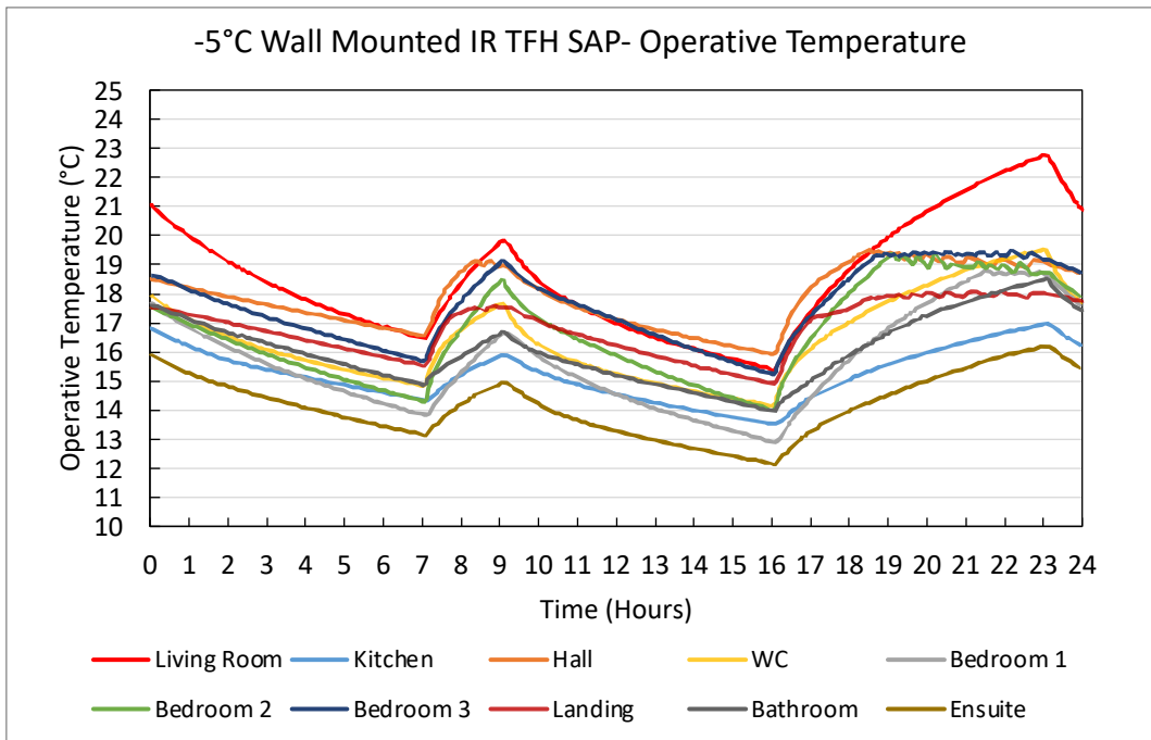
Figure 25. -5°C Wall Mounted IR TFH SAP - Operative Temperature Plots
