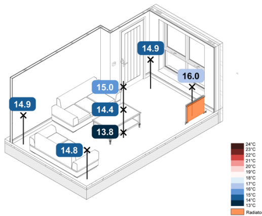
Figure 66. -5 °C Monobloc ASHP TFH Rads SAP – Spatial Air Temperatures
