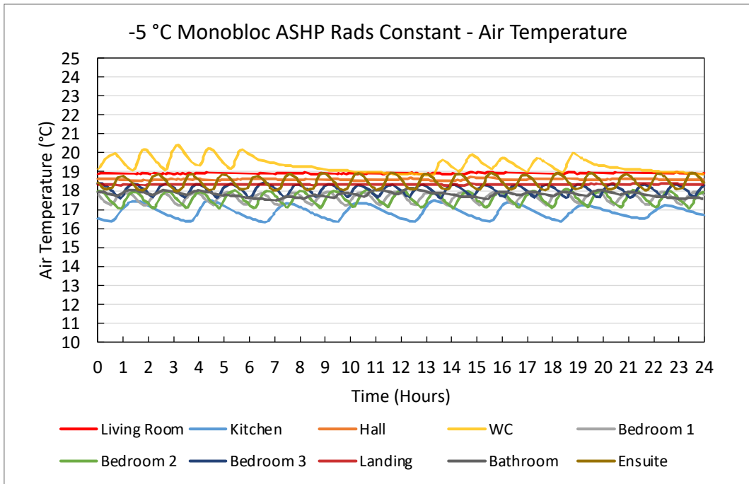
Figure 58. -5 °C Monobloc ASHP TFH Rads Constant – Air Temperature Plots
