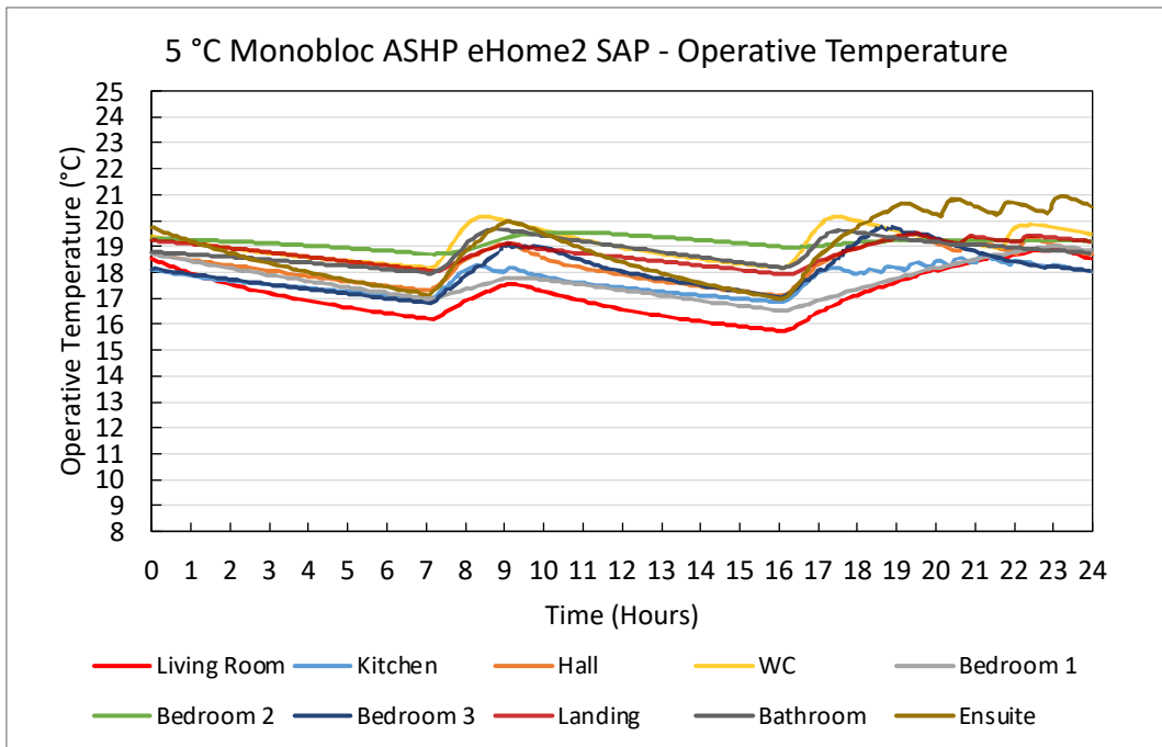
Figure 140. 5 °C Monobloc ASHP eHome2 SAP – Operative Temperature Plots
