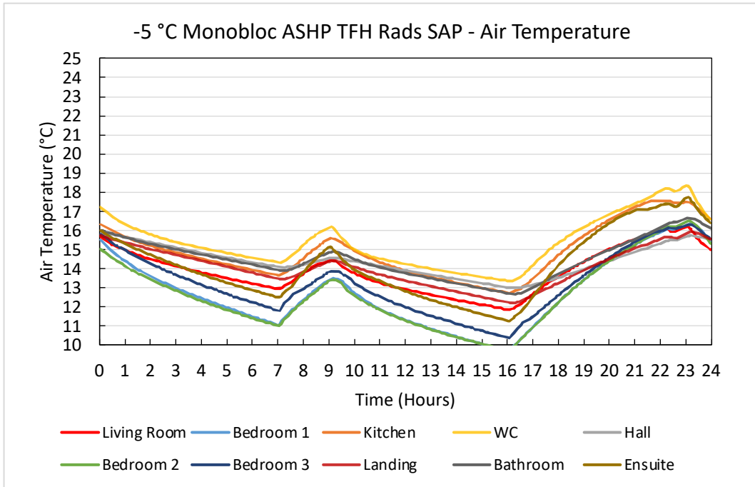
Figure 63. -5 °C Monobloc ASHP TFH Rads SAP – Air Temperature Plots
