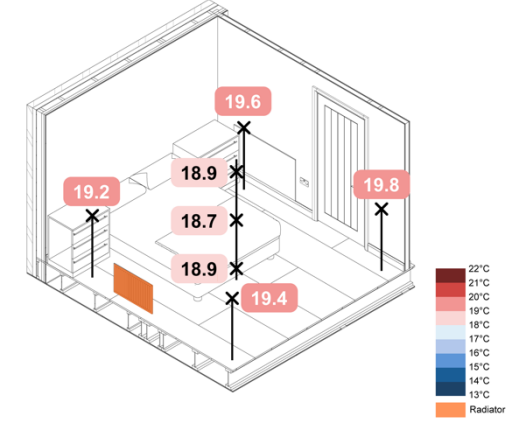
Figure 79. 5 °C Loft ASHP Rads + UFH Constant – Spatial Operative Temperatures
