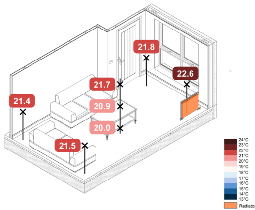
Figure 94. 5 °C Loft ASHP Rads SAP – Spatial Air Temperatures
