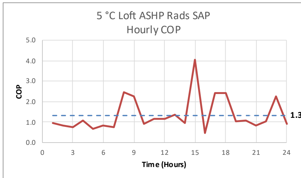
Figure 95. 5 °C Loft ASHP Rads SAP – Hourly COP
