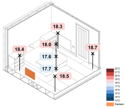
Figure 104. 5 °C Monobloc ASHP TFH Rads + UFH SAP – Spatial Air Temperatures
