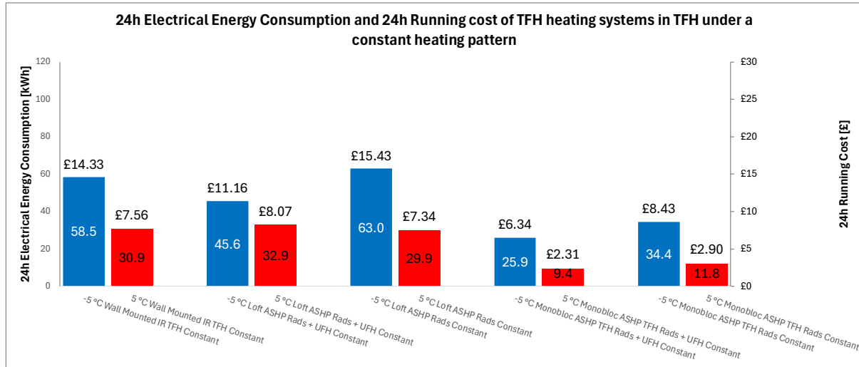
Figure 156. 24h Electrical Energy Consumption and 24h Running Cost of TFH heating system under a constant heating pattern
