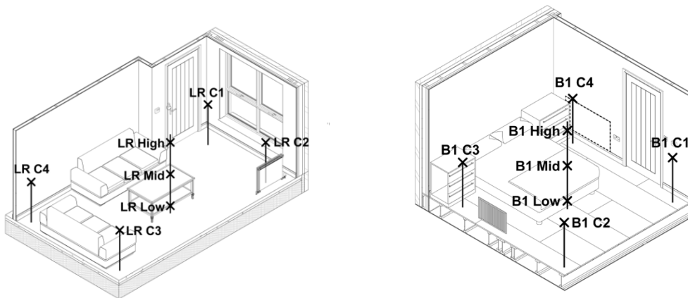
Figure 17. The Future Home Living Room (left) and Bedroom 1 (right) temperature measurement locations
