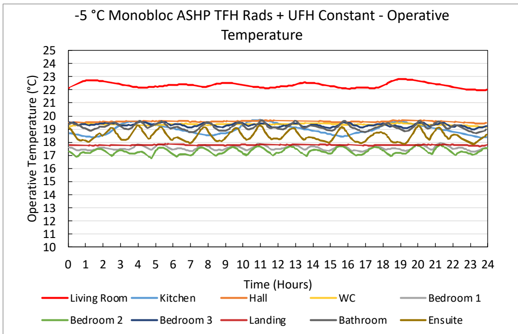
Figure 49. -5 °C Monobloc ASHP TFH Rads + UFH Constant – Operative Temperature Plots
