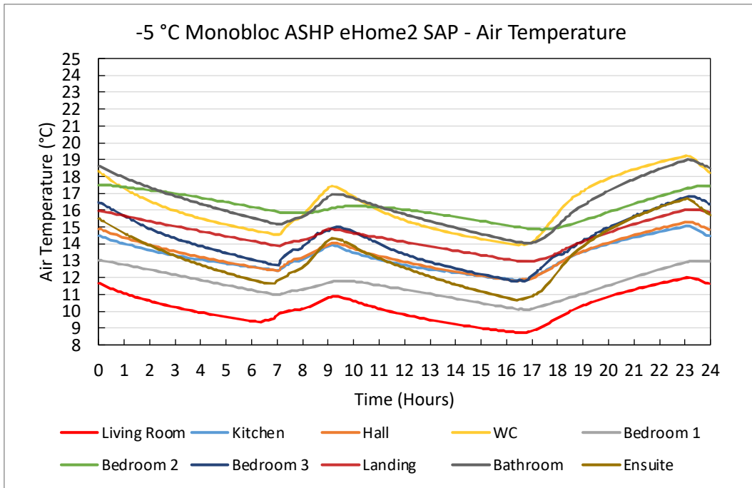
Figure 121. -5 °C Monobloc ASHP eHome2 SAP – Air Temperature Plots
