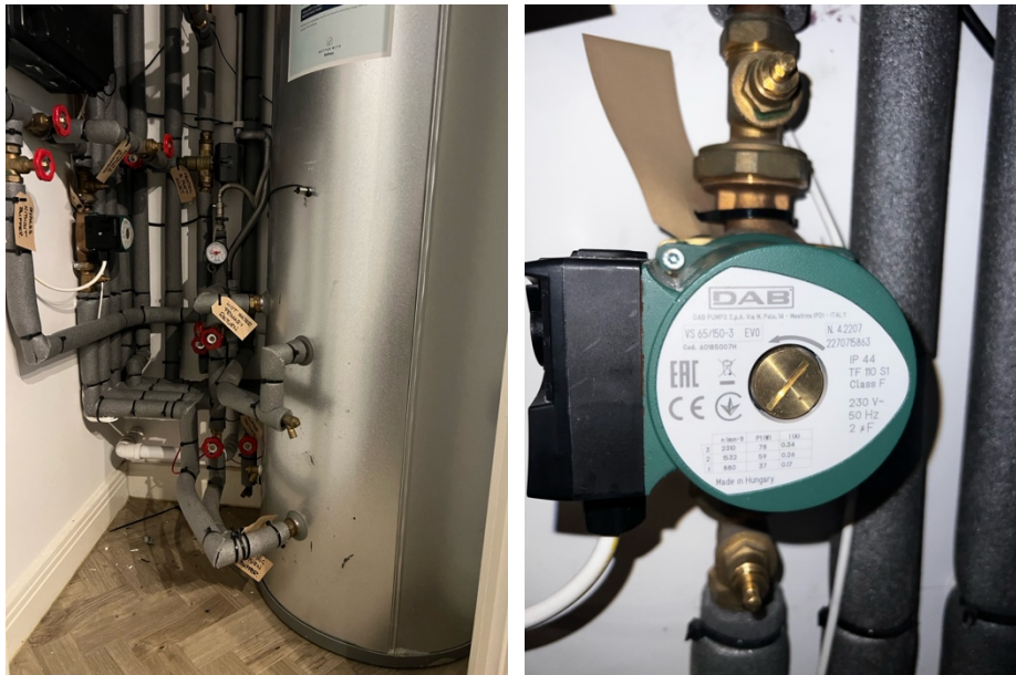
Figure 173. Buffer vessel and circulation pump
