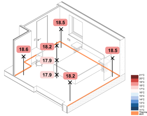
Figure 141. 5 °C Monobloc ASHP eHome2 SAP – Spatial Operative Temperatures
