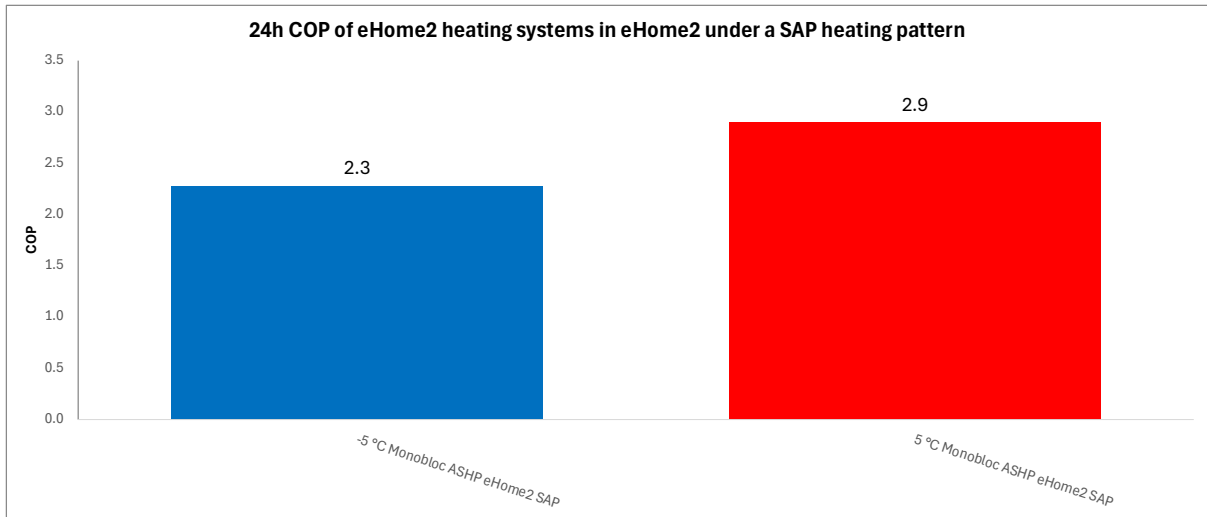
Figure 155. 24h COP of eHome2 heating systems under a SAP heating pattern
