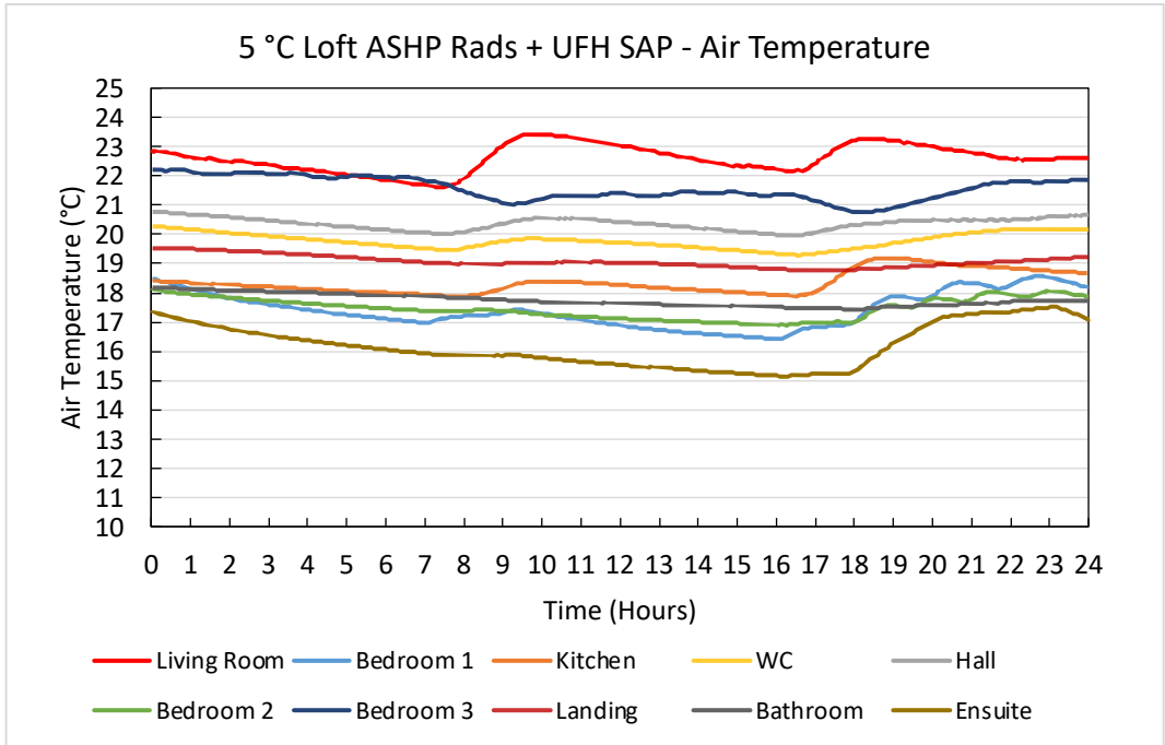
Figure 81. 5 °C Loft ASHP Rads + UFH SAP – Air Temperature Plots
