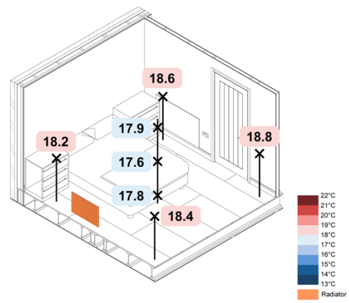
Figure 83. 5 °C Loft ASHP Rads + UFH SAP – Spatial Operative Temperatures
