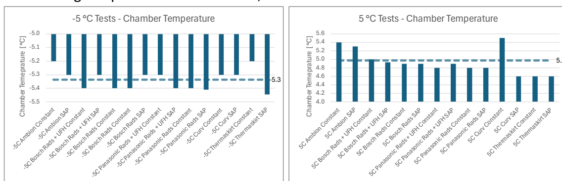
Figure 166. Chamber Temperatures in -5 °C and 5 °C tests
