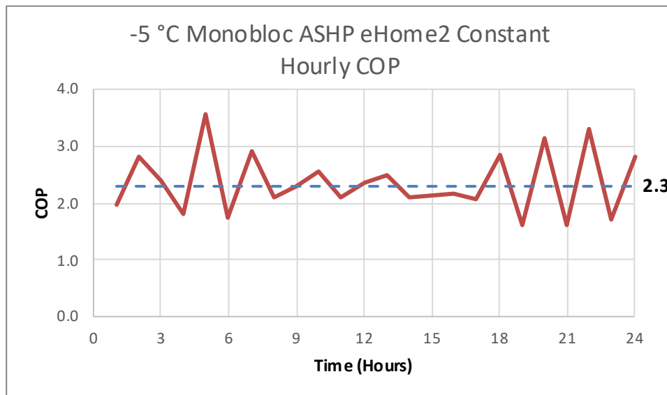
Figure 120. -5 °C Monobloc ASHP eHome2 Constant – Hourly COP
