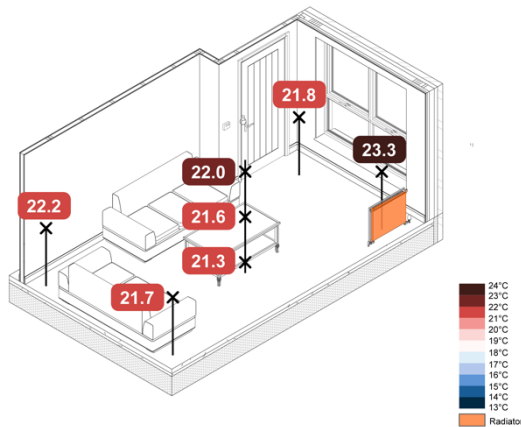
Figure 40. -5 °C Loft ASHP Rads Constant - Spatial Operative Temperatures
