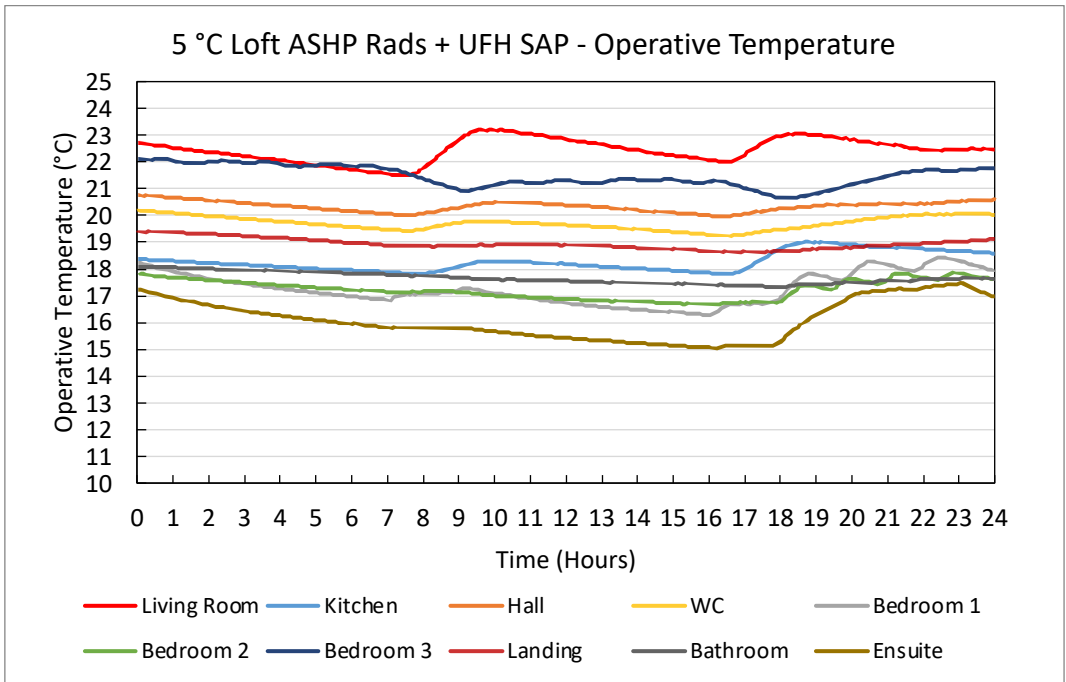
Figure 82. 5 °C Loft ASHP Rads + UFH SAP – Operative Temperature Plots
