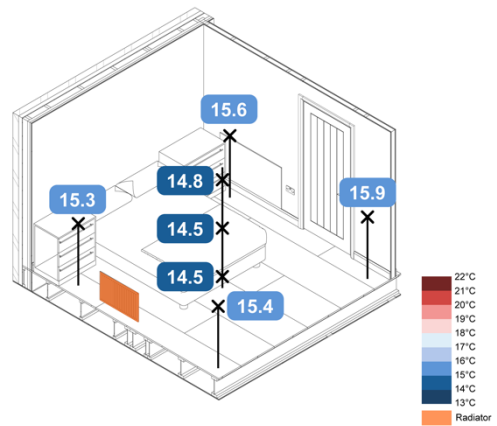
-5°C Loft ASHP Rads + UFH SAP – Operative - 7h
