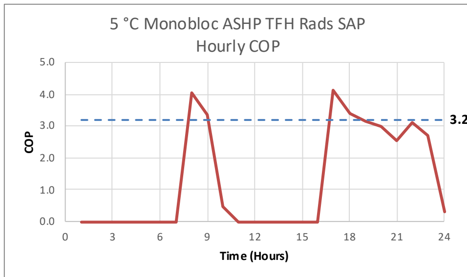
Figure 115. 5 °C Monobloc ASHP TFH Rads SAP – Hourly COP
