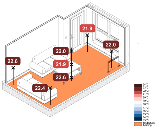
Figure 103. 5 °C Monobloc ASHP TFH Rads + UFH SAP – Spatial Operative Temperatures
