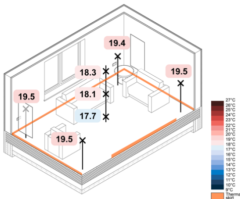
Figure 119. -5 °C Monobloc ASHP eHome2 Constant – Operative Temperature Plots
