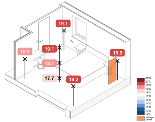
Figure 150. 5 °C Wall Mounted eHome2 SAP – Spatial Air Temperatures
