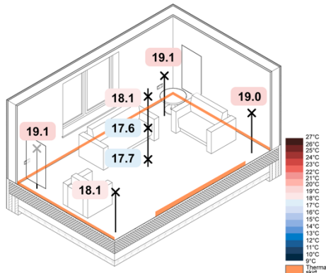
Figure 142. 5 °C Monobloc ASHP eHome2 SAP – Spatial Air Temperatures
