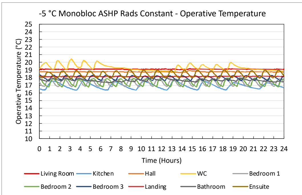
Figure 59. -5 °C Monobloc ASHP TFH Rads Constant – Operative Temperature Plots
