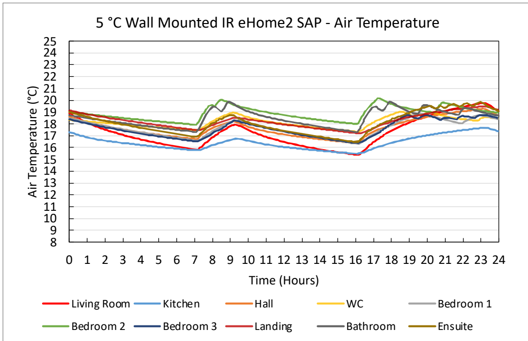
Figure 148. 5 °C Wall Mounted eHome2 SAP – Air Temperature Plots
