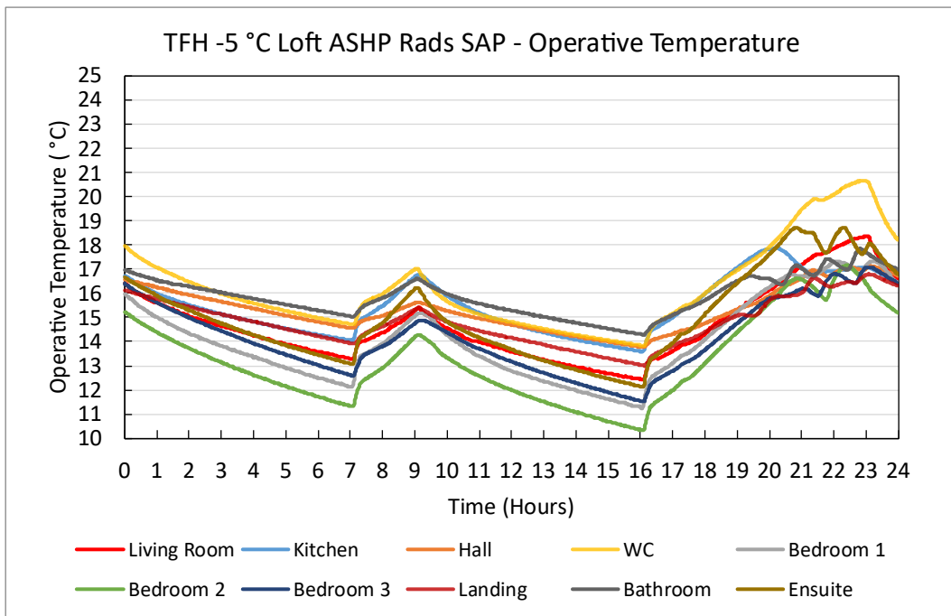
Figure 44. -5 °C Loft ASHP Rads SAP – Operative Temperature Plots
