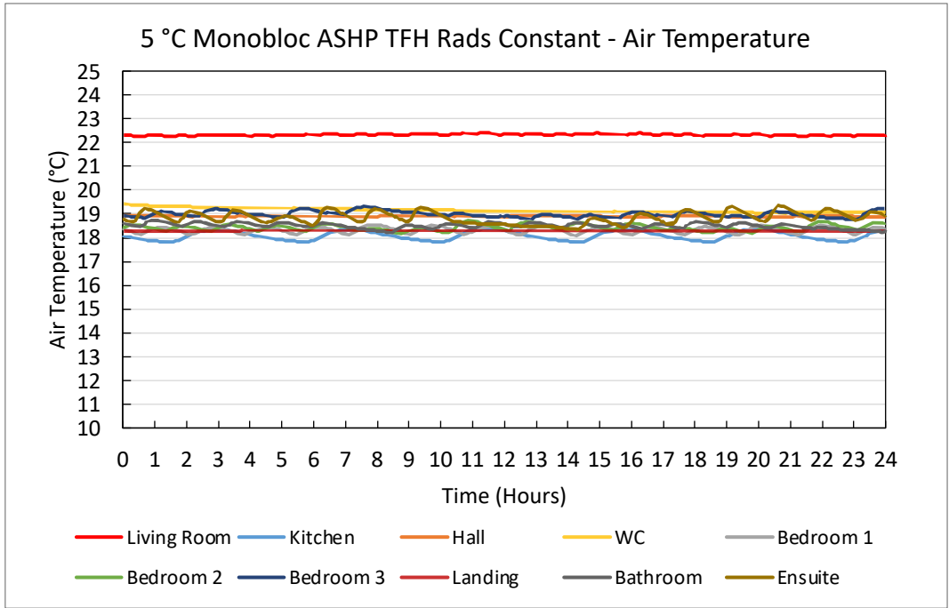
Figure 106. 5 °C Monobloc ASHP TFH Rads Constant – Air Temperature Plots
