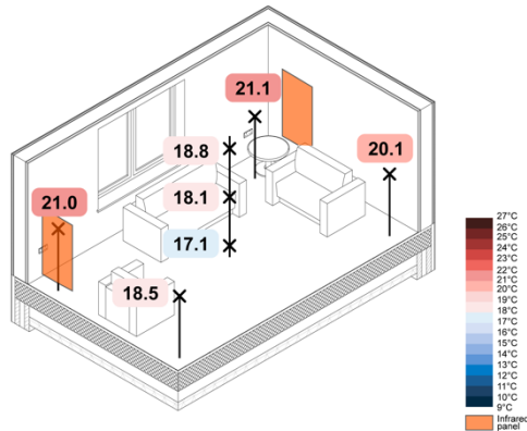
Figure 150. 5 °C Wall Mounted eHome2 SAP – Spatial Air Temperatures
