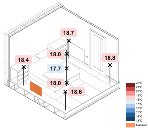
Figure 98. 5 °C Monobloc ASHP TFH Rads + UFH Constant – Spatial Operative Temperatures
