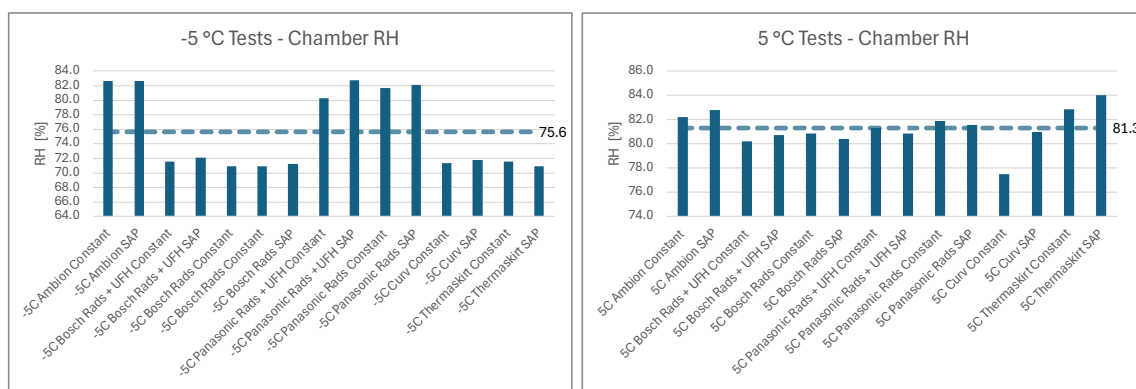
Figure 165. Chamber Humidity in -5 °C and 5 °C tests
