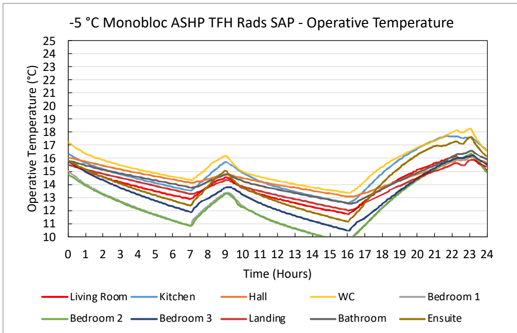
Figure 64. -5 °C Monobloc ASHP TFH Rads SAP – Operative Temperature Plots
