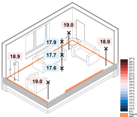
Figure 141. 5 °C Monobloc ASHP eHome2 SAP – Spatial Operative Temperatures
