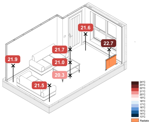
Figure 93. 5 °C Loft ASHP Rads SAP – Spatial Operative Temperatures
