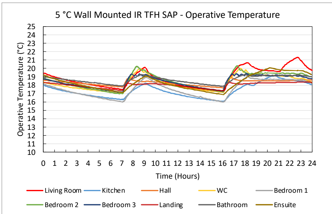
Figure 73. 5 °C Wall Mounted IR TFH SAP – Operative Temperature Plots
