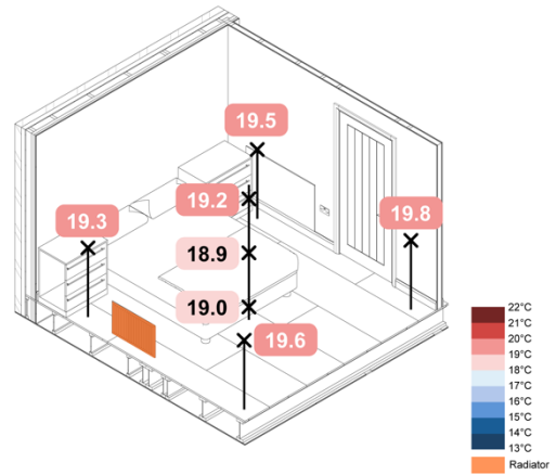
Figure 78. 5 °C Loft ASHP Rads + UFH Constant – Spatial Air Temperatures
