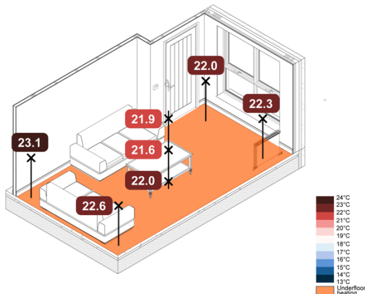
Figure 31. -5°C Loft ASHP Rads + UFH Constant - Spatial Operative Temperature Plots
