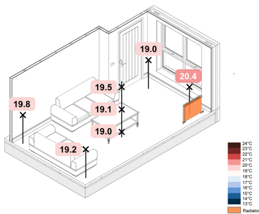
Figure 60. -5 °C Monobloc ASHP TFH Rads Constant – Spatial Operative Temperatures
