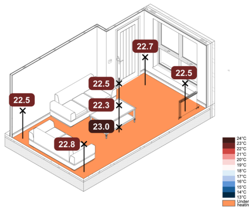
Figure 104. 5 °C Monobloc ASHP TFH Rads + UFH SAP – Spatial Air Temperatures
