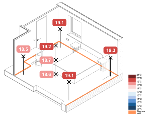
Figure 137. 5 °C Monobloc ASHP eHome2 Constant – Spatial Air Temperatures
