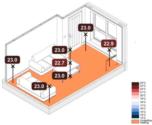
Figure 78. 5 °C Loft ASHP Rads + UFH Constant – Spatial Air Temperatures
