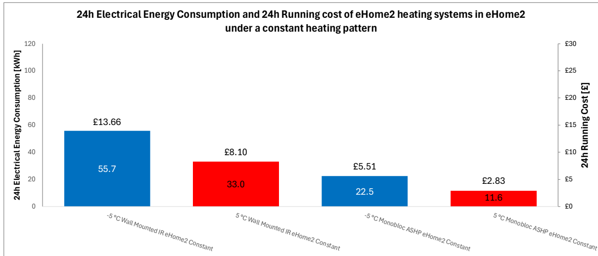
Figure 158. 24h Electrical Energy Consumption and 24h Running Cost of eHome2 heating system under a constant heating pattern
