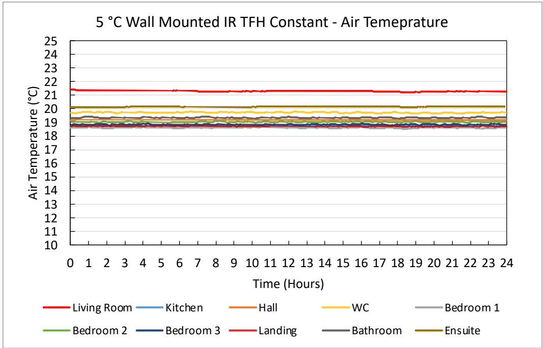
Figure 68. 5°C Wall Mounted IR TFH Constant – Air Temperature Plots
