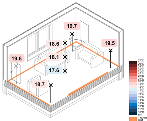
Figure 118. -5 °C Monobloc ASHP eHome2 Constant – Spatial Air Temperatures
