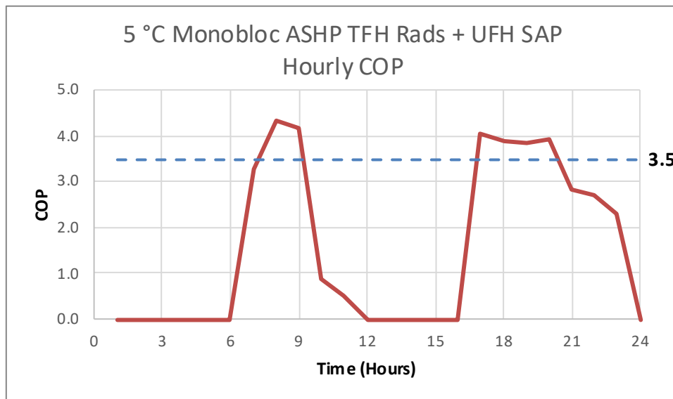
Figure 105. 5 °C Monobloc ASHP TFH Rads + UFH SAP – Hourly COP
