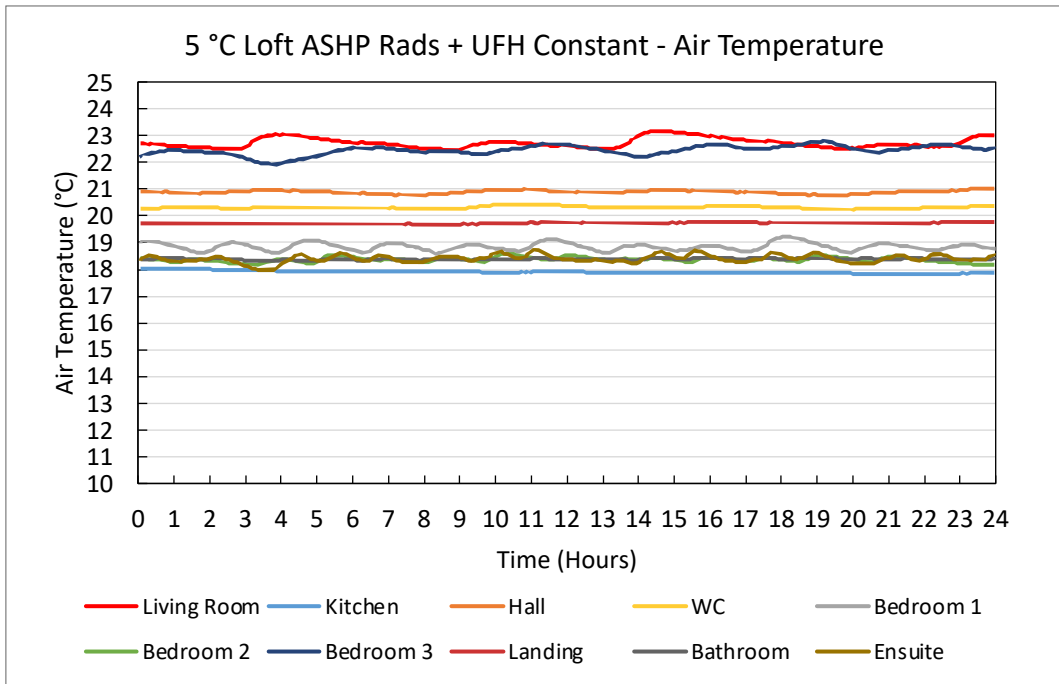
Figure 76. 5 °C Loft ASHP Rads + UFH Constant – Air Temperature Plots
