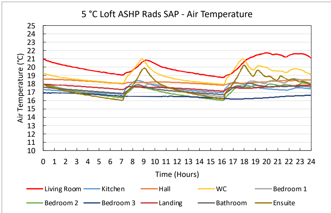
Figure 91. 5 °C Loft ASHP Rads SAP – Air Temperature Plots
