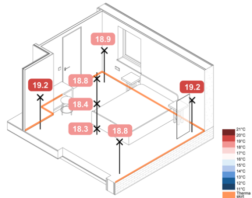
Figure 119. -5 °C Monobloc ASHP eHome2 Constant – Operative Temperature Plots
