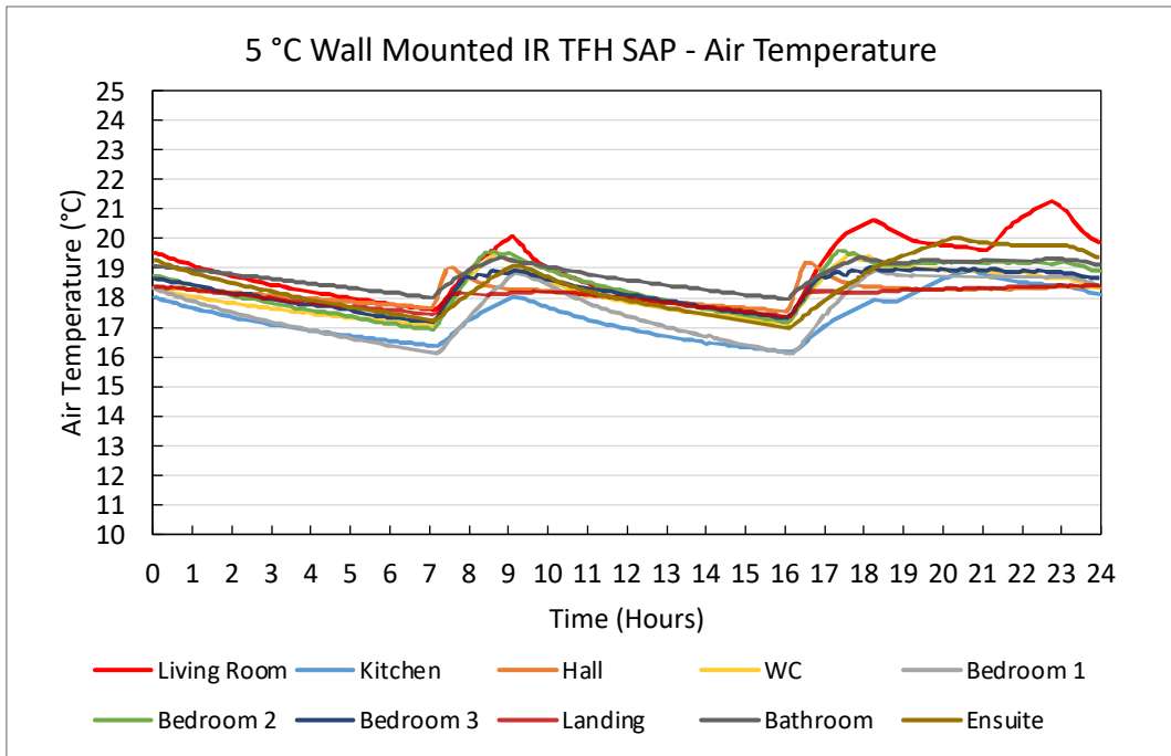
Figure 72. 5 °C Wall Mounted IR TFH SAP – Air Temperature Plots
