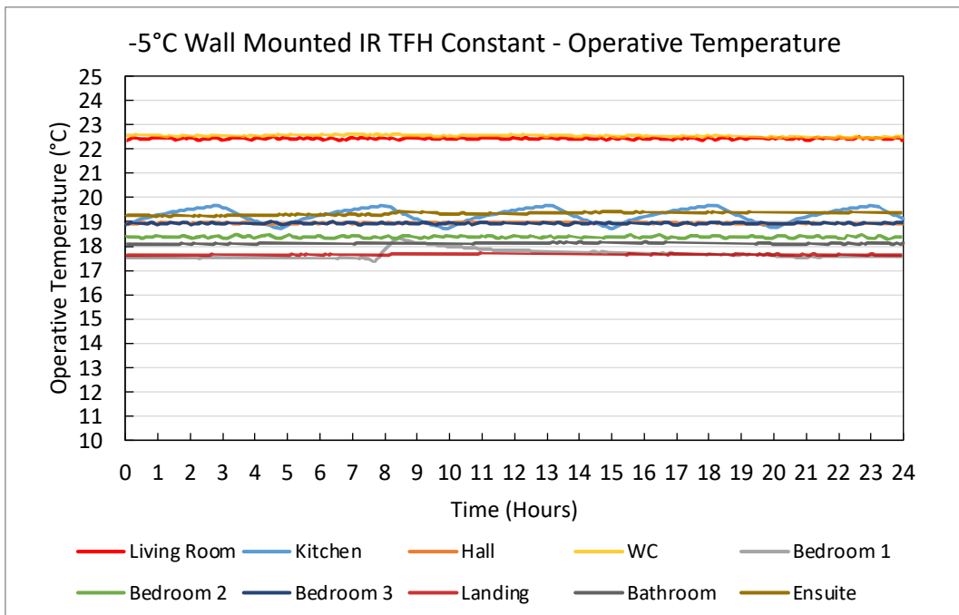
Figure 21. -5°C Wall Mounted IR TFH Constant Operative Temperature Plot
