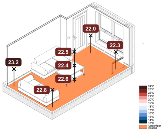
Figure 50. -5 °C Monobloc ASHP TFH Rads + UFH Constant – Spatial Operative Temperatures
