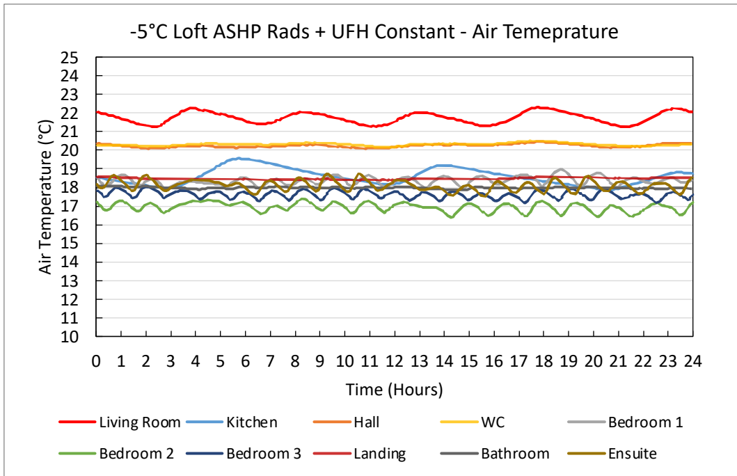
Figure 28. -5°C Loft ASHP Rads + UFH Constant - Air Temperature Plot
