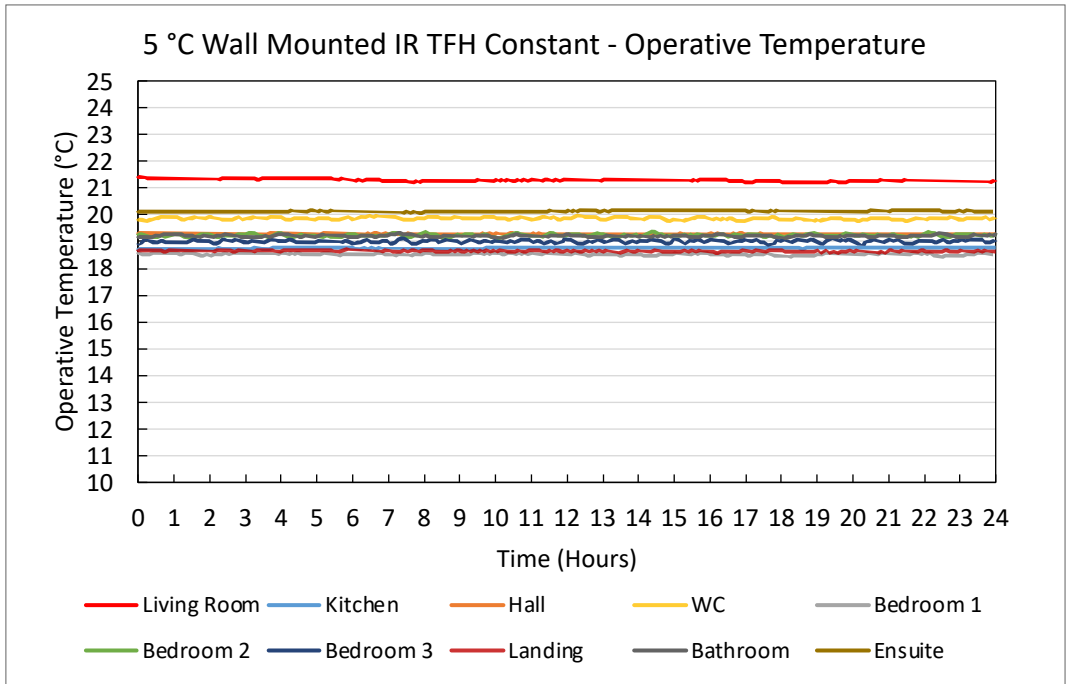
Figure 69. 5°C Wall Mounted IR TFH Constant – Operative Temperature Plots
