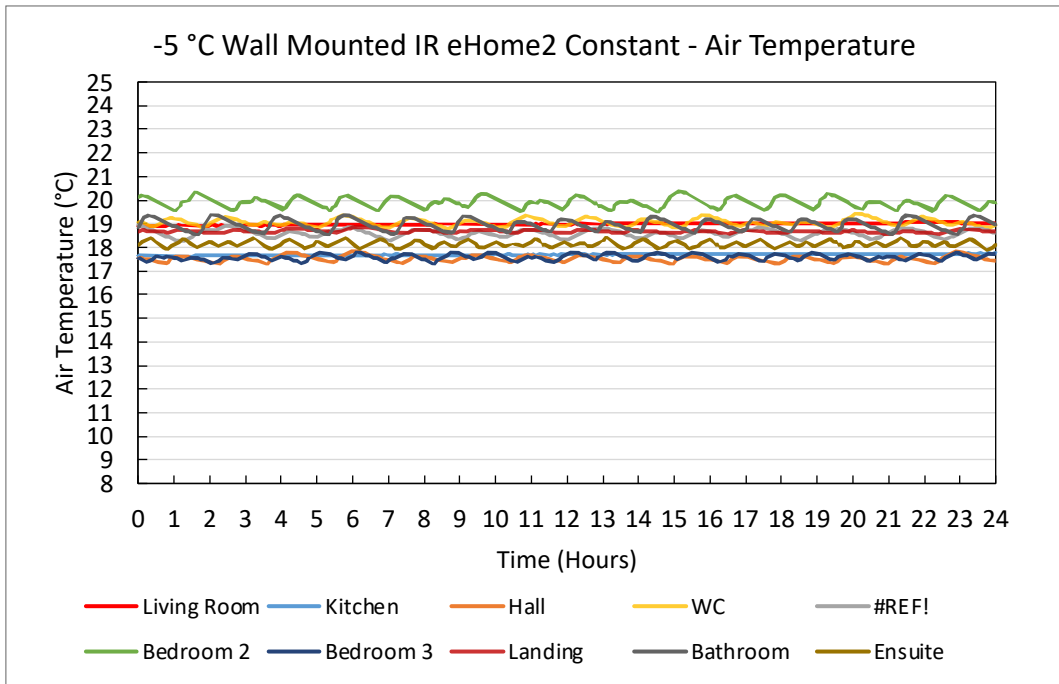
Figure 126. -5 °C Wall Mounted IR eHome2 Constant – Air Temperature Plots
