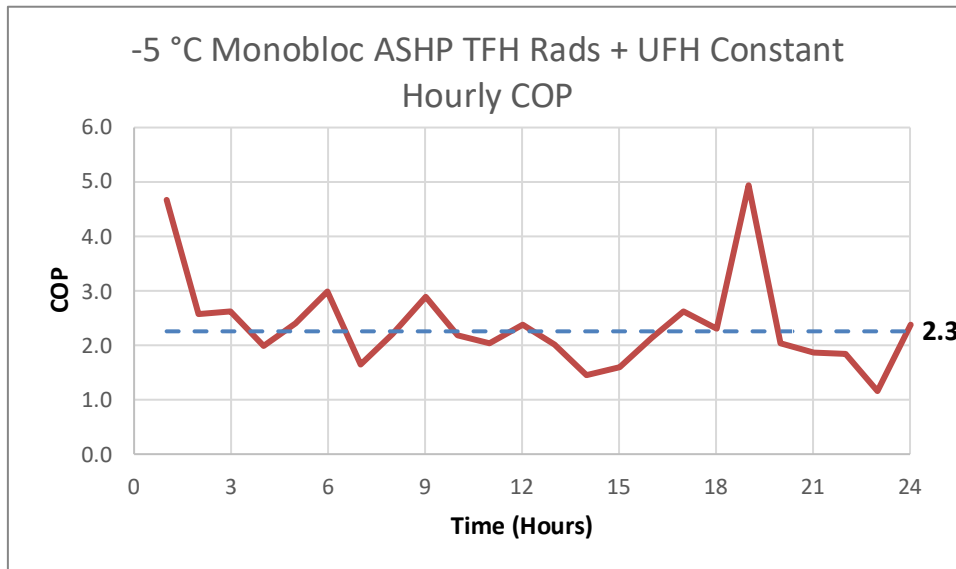
Figure 52. -5 °C Monobloc ASHP TFH Rads + UFH Constant – Hourly COP
