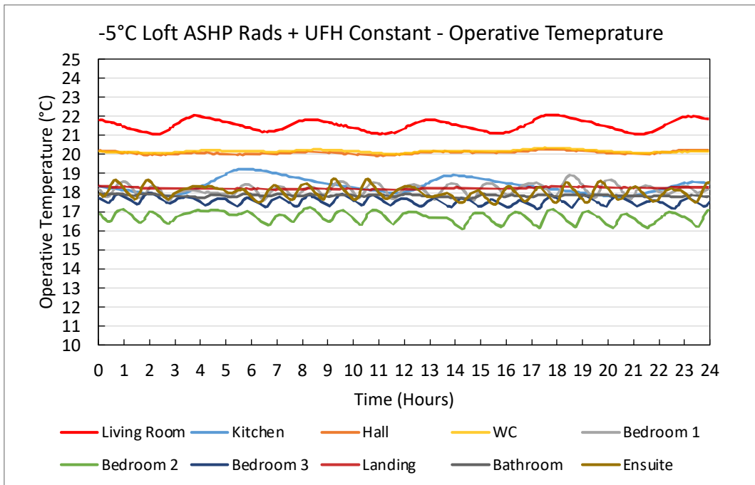
Figure 29. -5°C Loft ASHP Rads + UFH Constant - Operative Temperature Plot
