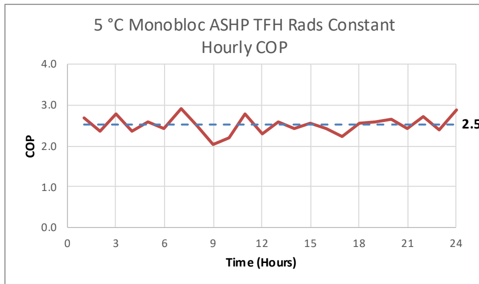
Figure 110. 5 °C Monobloc ASHP TFH Rads Constant – Hourly COP
