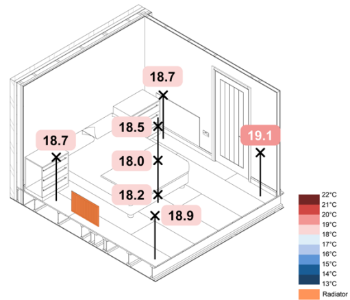
Figure 94. 5 °C Loft ASHP Rads SAP – Spatial Air Temperatures
