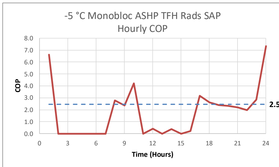
Figure 67. -5 °C Monobloc ASHP TFH Rads SAP – Hourly COP
