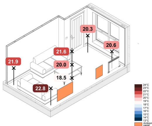
-5°C Wall Mounted IR TFH SAP – Operative - 7h
