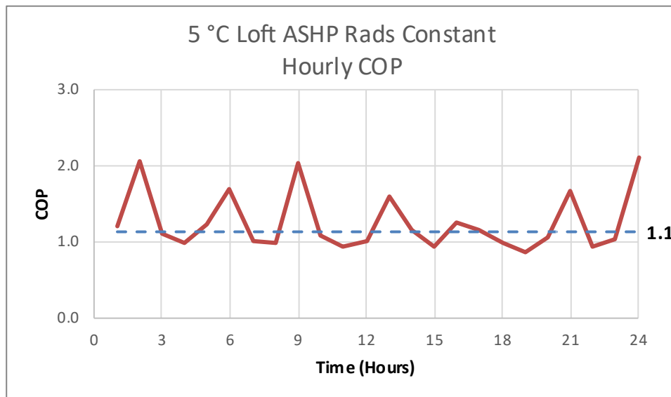
Figure 90. 5 °C Loft ASHP Rads Constant – Hourly COP
