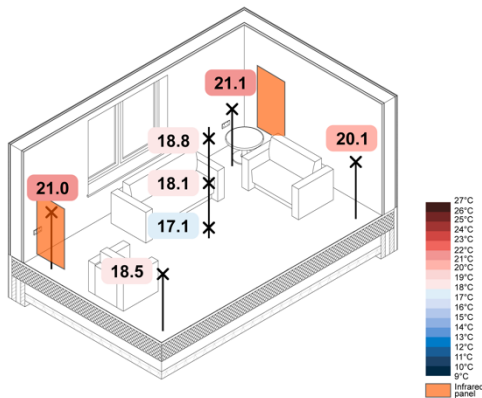
Figure 128. -5 °C Wall Mounted IR eHome2 Constant – Spatial Air Temperatures
