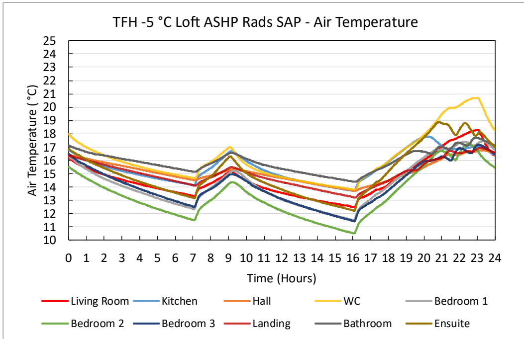
Figure 43. -5 °C Loft ASHP Rads SAP – Air Temperature Plots
