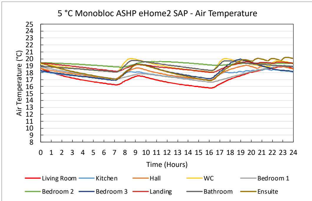
Figure 139. 5 °C Monobloc ASHP eHome2 SAP – Air Temperature Plots
