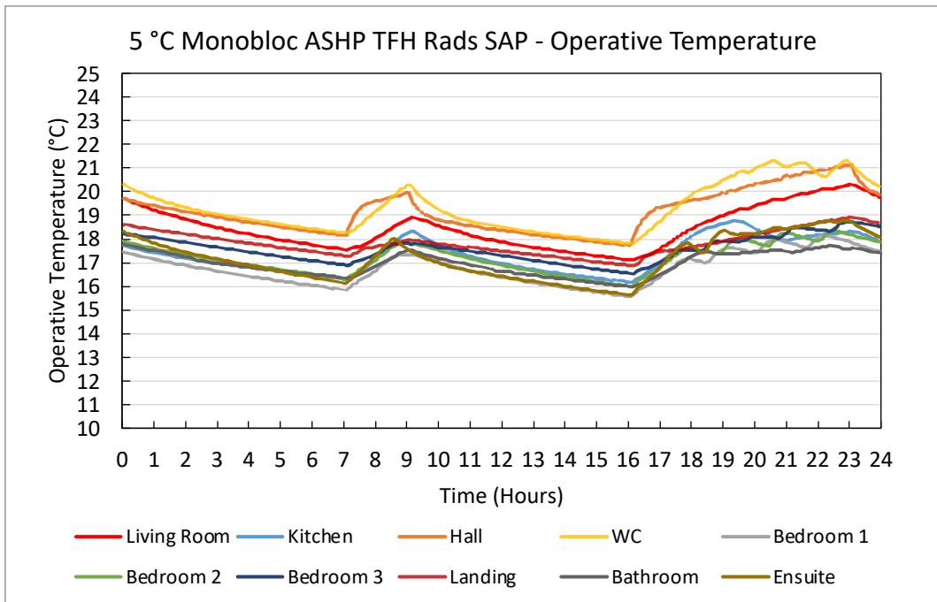
Figure 112. 5 °C Monobloc ASHP TFH Rads SAP – Operative Temperature Plots
