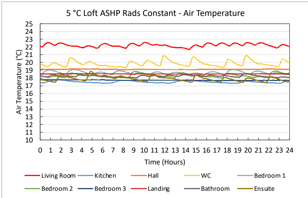
Figure 86. 5 °C Loft ASHP Rads Constant – Air Temperature Plots
