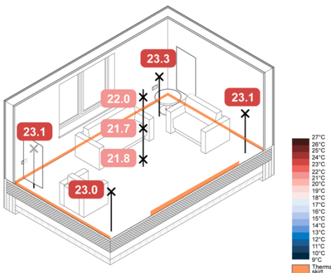
Figure 136. 5 °C Monobloc ASHP eHome2 Constant – Operative Temperature Plots
