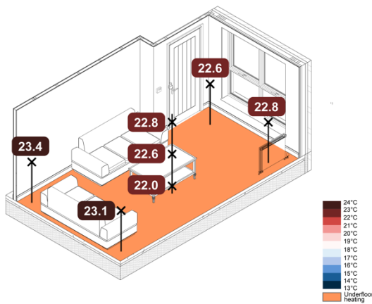
Figure 83. 5 °C Loft ASHP Rads + UFH SAP – Spatial Operative Temperatures
