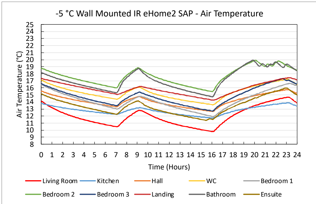
Figure 130. -5 °C Wall Mounted IR eHome2 SAP – Air Temperature Plots
