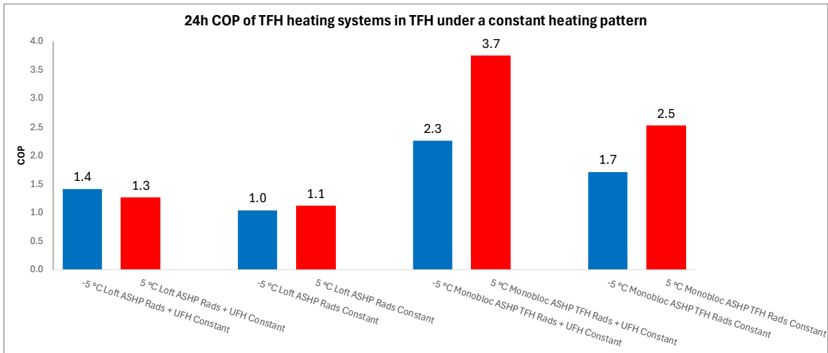
Figure 152. 24h COP of TFH heating systems under a constant heating pattern
