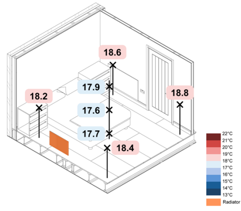
Figure 40. -5 °C Loft ASHP Rads Constant - Spatial Operative Temperatures
