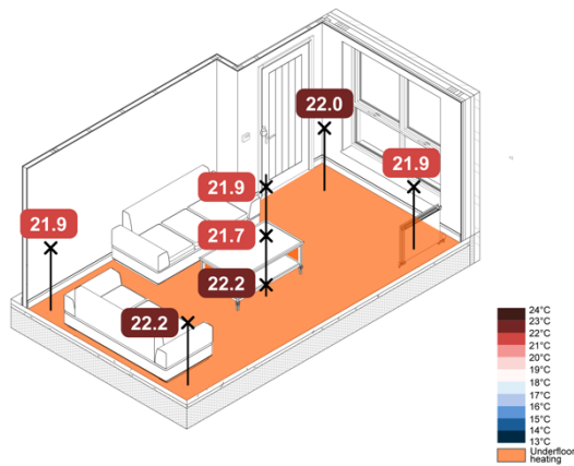
Figure 99. 5 °C Monobloc ASHP TFH Rads + UFH Constant – Spatial Air Temperatures
