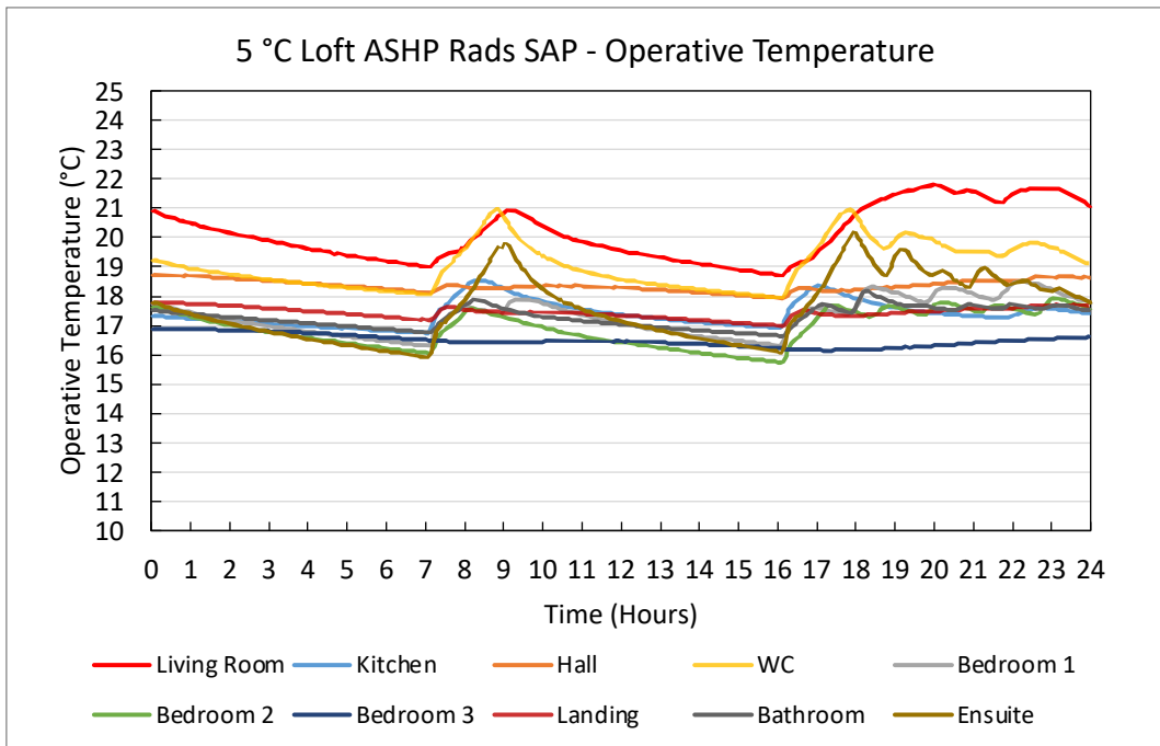
Figure 92. 5 °C Loft ASHP Rads SAP – Operative Temperature Plots
