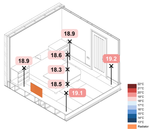
Figure 109. 5 °C Monobloc ASHP TFH Rads Constant – Spatial Air Temperatures
