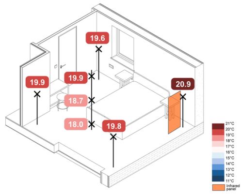
-5 °C Wall Mounted IR eHome2 Constant – Operative - 7h
