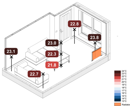
Figure 108. 5 °C Monobloc ASHP TFH Rads Constant – Spatial Operative Temperatures
