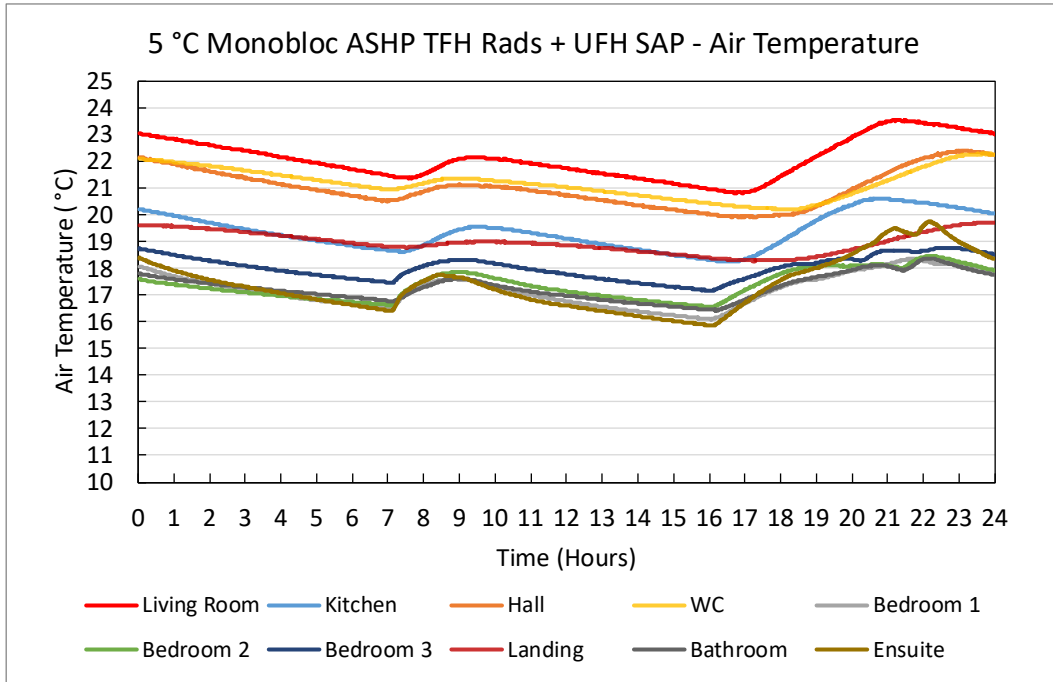
Figure 101. 5 °C Monobloc ASHP TFH Rads + UFH SAP – Air Temperature Plots
