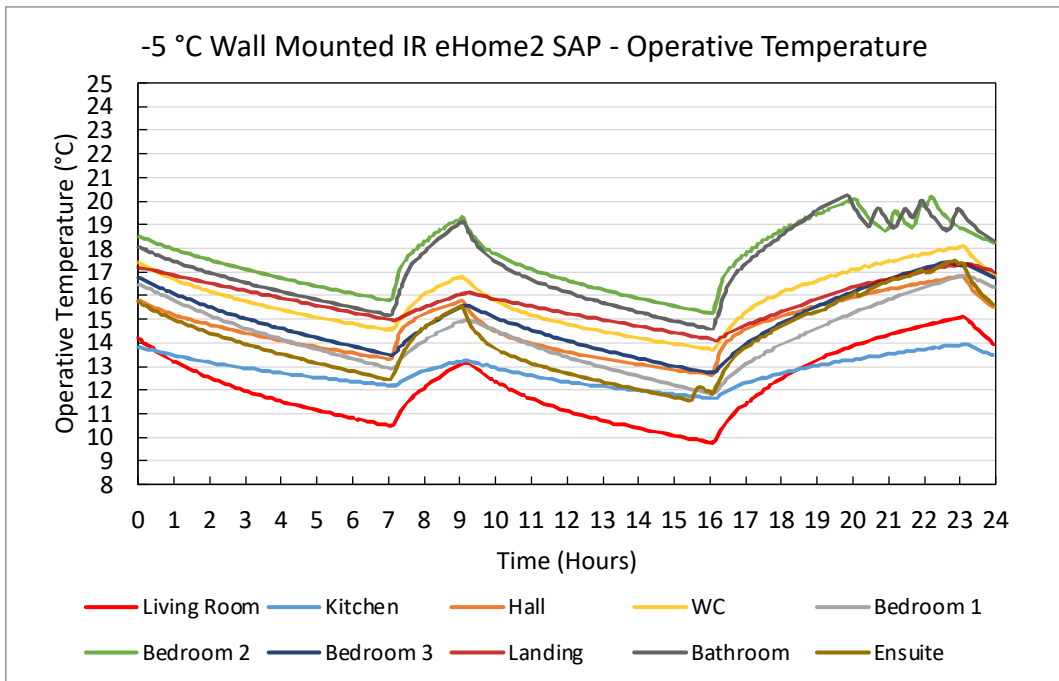
Figure 131. -5 °C Wall Mounted IR eHome2 SAP – Operative Temperature Plots
