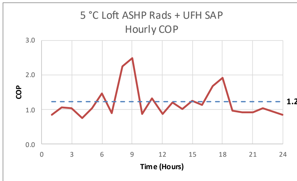
Figure 85. 5 °C Loft ASHP Rads + UFH SAP – Hourly COP
