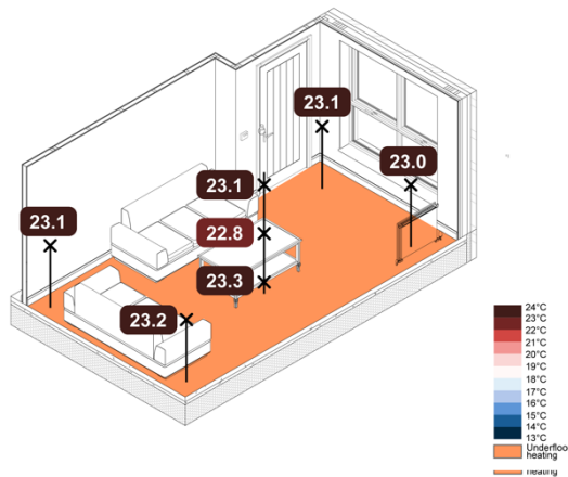
Figure 84. 5 °C Loft ASHP Rads + UFH SAP – Spatial Air Temperatures
