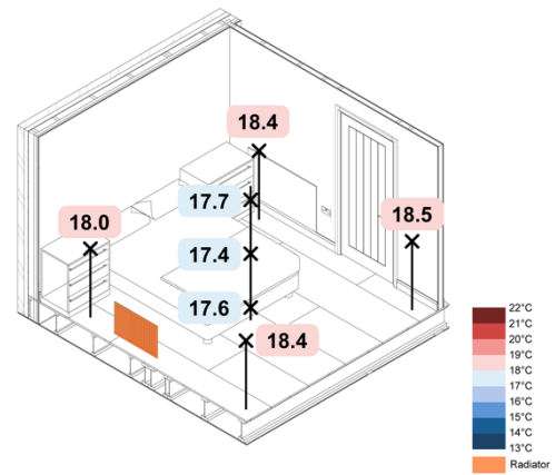
Figure 60. -5 °C Monobloc ASHP TFH Rads Constant – Spatial Operative Temperatures
