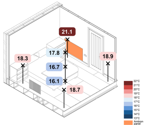
-5°C Wall Mounted IR TFH SAP – Air - 7h
