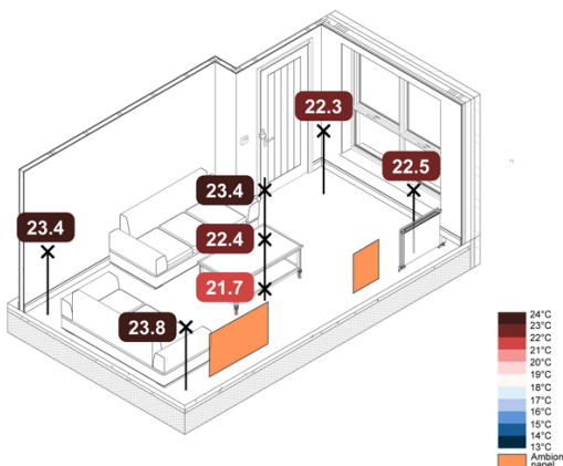
-5°C Wall Mounted IR TFH Constant – Operative - 7h
