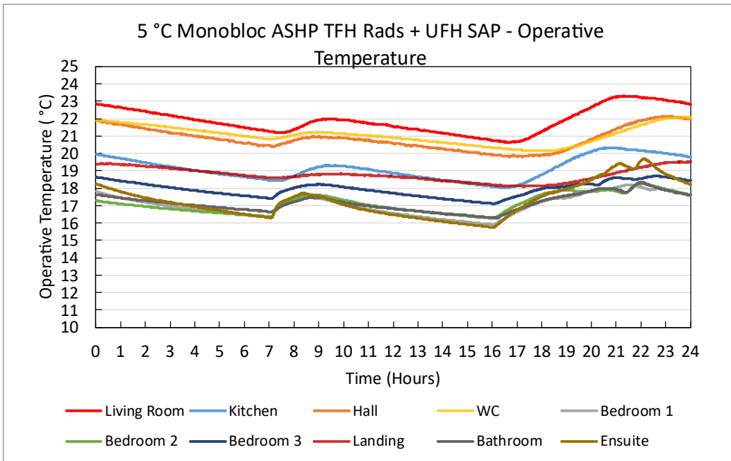
Figure 102. 5 °C Monobloc ASHP TFH Rads + UFH SAP – Operative Temperature Plots
