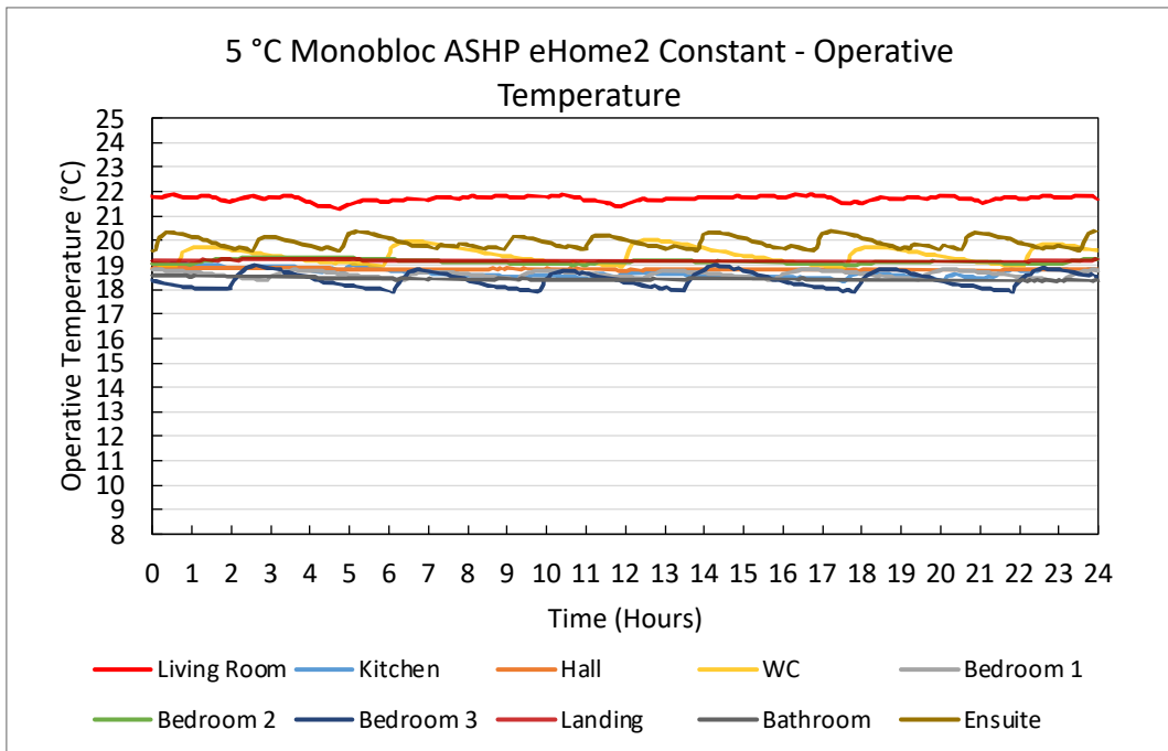
Figure 135. 5 °C Monobloc ASHP eHome2 Constant – Operative Temperature Plots
