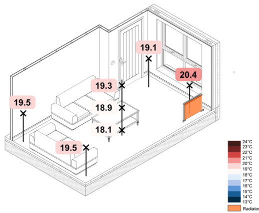
Figure 61. -5 °C Monobloc ASHP TFH Rads Constant – Spatial Air Temperatures
