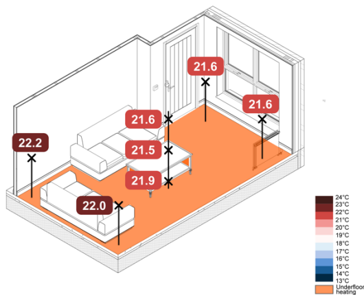
Figure 98. 5 °C Monobloc ASHP TFH Rads + UFH Constant – Spatial Operative Temperatures
