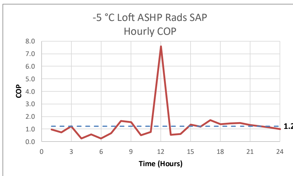
Figure 47. -5 °C Loft ASHP Rads SAP – Hourly COP
