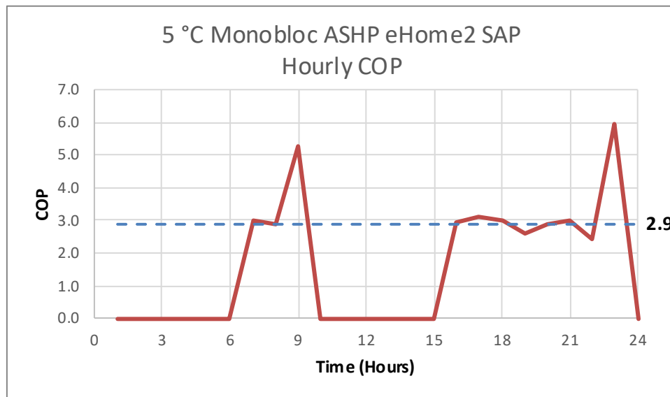
Figure 143. 5 °C Monobloc ASHP eHome2 SAP – Hourly COP
