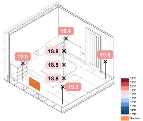
5 °C Loft ASHP Rads Constant – Operative - 7h
