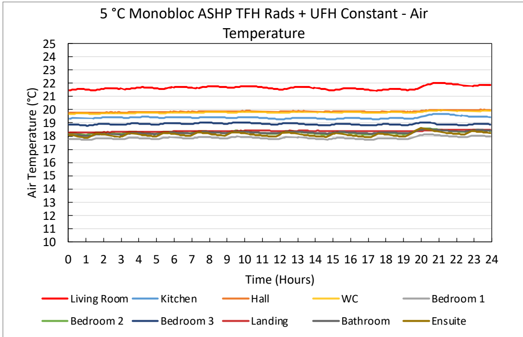
Figure 96. 5 °C Monobloc ASHP TFH Rads + UFH Constant – Air Temperature Plots
