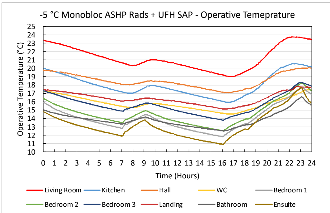
Figure 54. -5 °C Monobloc ASHP TFH Rads + UFH SAP – Operative Temperature Plots
