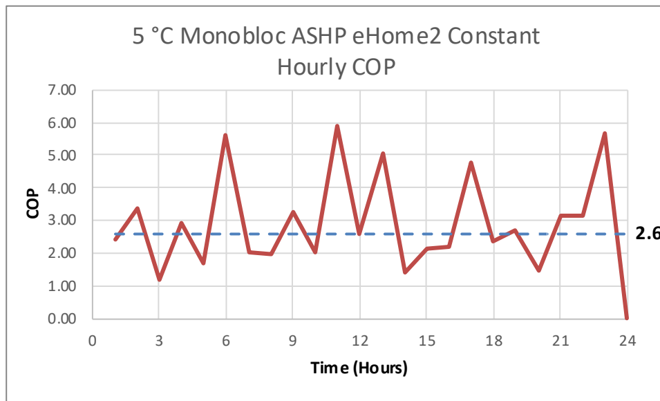
Figure 138. 5 °C Monobloc ASHP eHome2 Constant – Hourly COP
