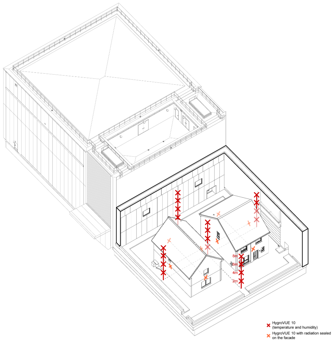
Figure 14. Diagram of air temperature and humidity sensor locations within the chambers
