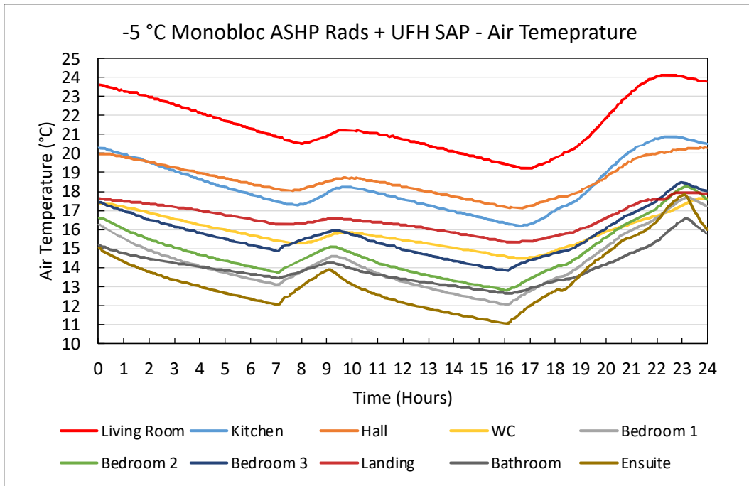
Figure 53. -5 °C Monobloc ASHP TFH Rads + UFH SAP – Air Temperature Plots
