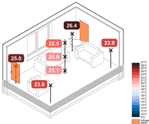
Figure 146. 5 °C Wall Mounted eHome2 Constant – Spatial Operative Temperatures
