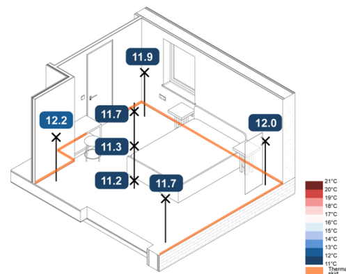
-5 °C Monobloc ASHP eHome2 SAP – Operative - 7h
