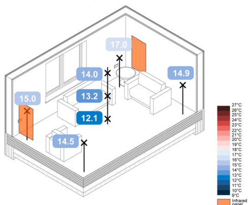
Figure 133. -5 °C Wall Mounted IR eHome2 SAP – Spatial Operative Temperatures
