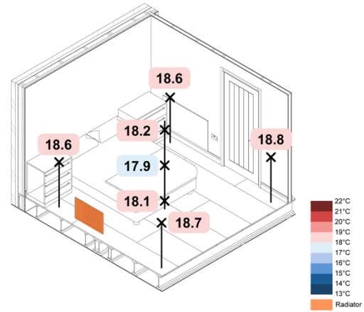
Figure 99. 5 °C Monobloc ASHP TFH Rads + UFH Constant – Spatial Air Temperatures
