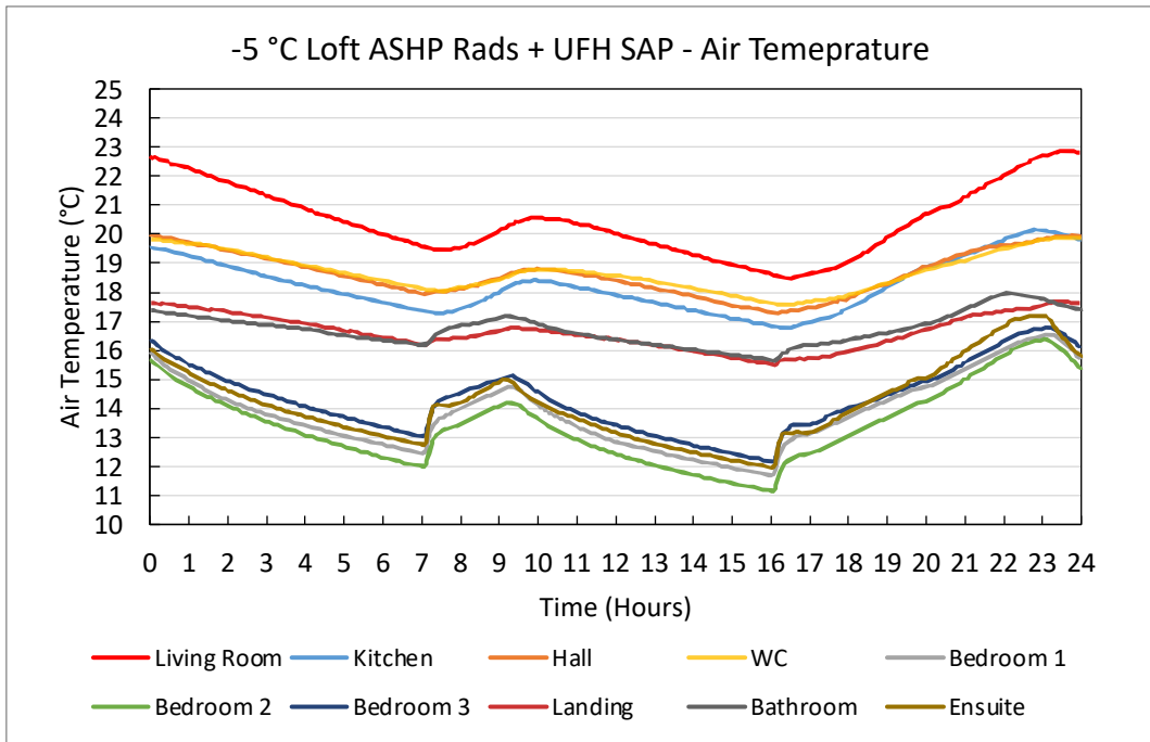
Figure 33. -5°C Loft ASHP Rads + UFH SAP – Air Temperature Plots
