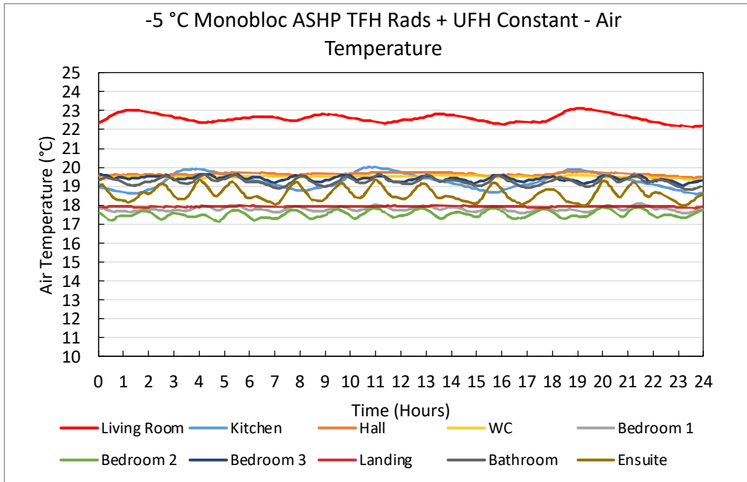
Figure 48. -5 °C Monobloc ASHP TFH Rads + UFH Constant – Air Temperature Plots
