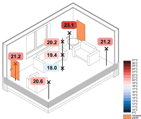
-5 °C Wall Mounted IR eHome2 Constant – Operative - 7h
