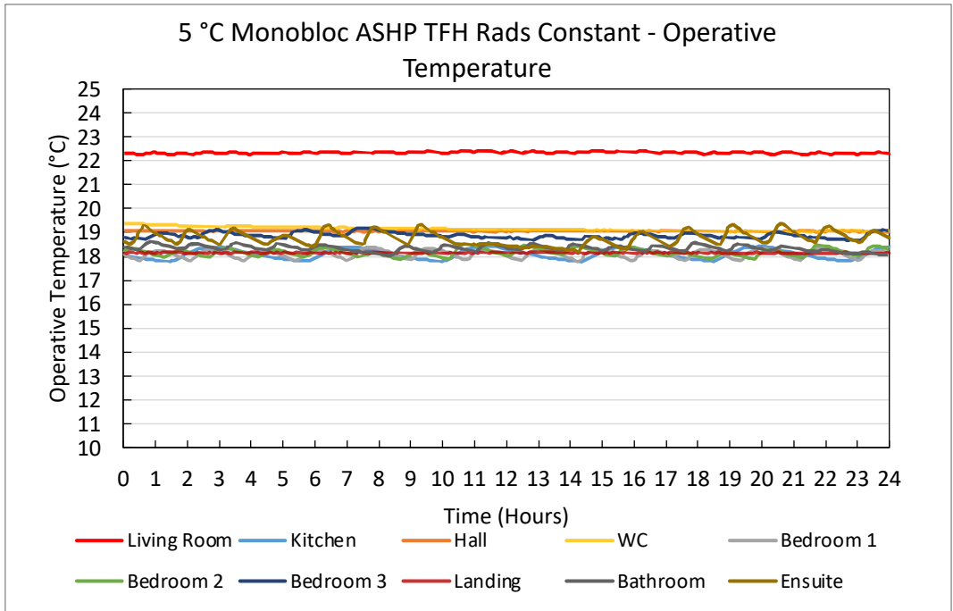
Figure 107. 5 °C Monobloc ASHP TFH Rads Constant – Operative Temperature Plots
