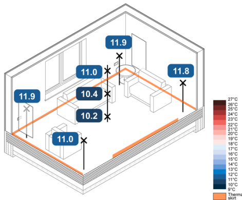
-5 °C Monobloc ASHP eHome2 SAP – Air - 7h
