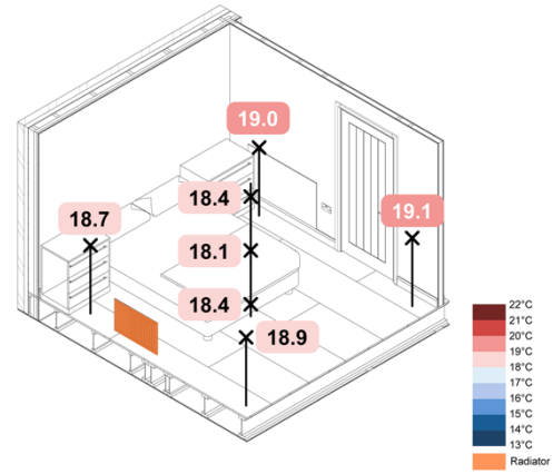
Figure 108. 5 °C Monobloc ASHP TFH Rads Constant – Spatial Operative Temperatures
