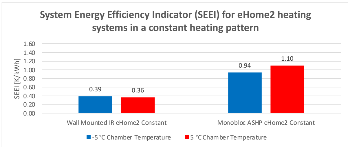
Figure 162. System Energy Efficiency Indicator (SEEI) for eHome2 heating system in a constant heating pattern
