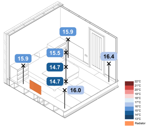
Figure 56. -5 °C Monobloc ASHP TFH Rads + UFH SAP – Spatial Air Temperatures
