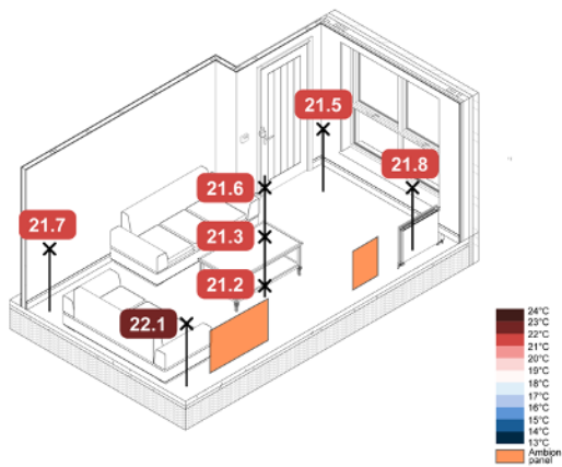
Figure 70. 5°C Wall Mounted IR TFH Constant – Spatial Air Temperatures
