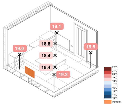
-5°C Loft ASHP Rads + UFH Constant – Air - 7h
