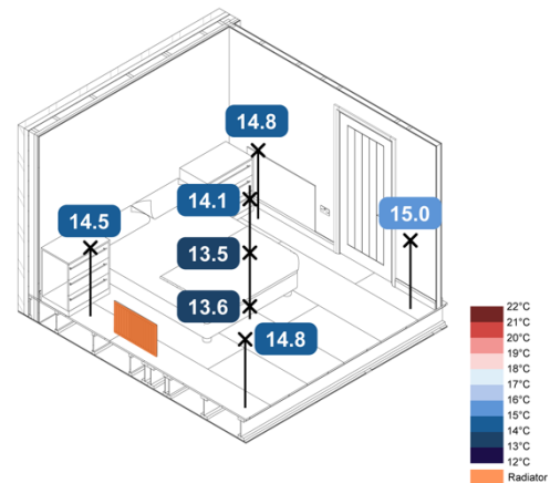
Figure 65. -5 °C Monobloc ASHP TFH Rads SAP – Spatial Operative Temperatures
