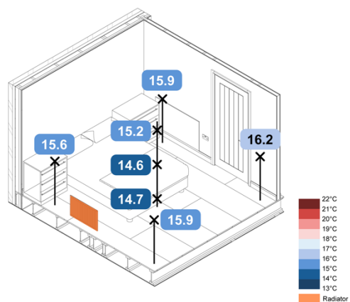
Figure 55. -5 °C Monobloc ASHP TFH Rads + UFH SAP – Spatial Operative Temperatures
