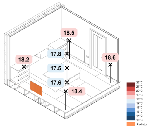
Figure 103. 5 °C Monobloc ASHP TFH Rads + UFH SAP – Spatial Operative Temperatures
