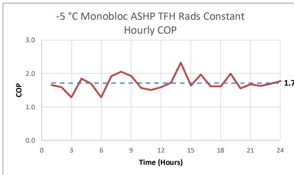
Figure 62. -5 °C Monobloc ASHP TFH Rads Constant – Hourly COP
