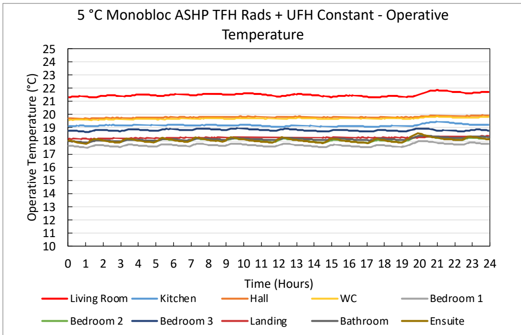
Figure 97. 5 °C Monobloc ASHP TFH Rads + UFH Constant – Operative Temperature Plots
