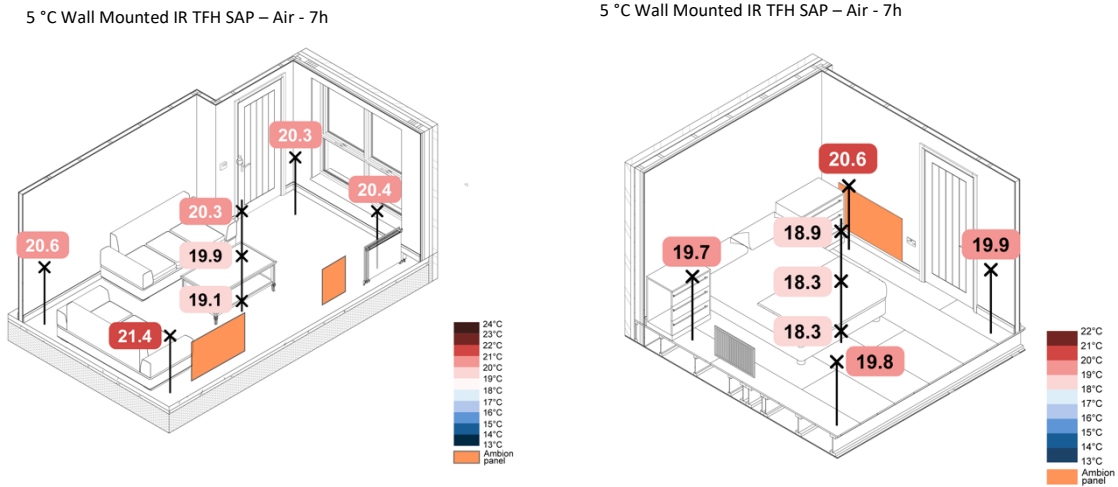
Figure 75. 5 °C Wall Mounted IR TFH SAP – Spatial Air Temperatures
